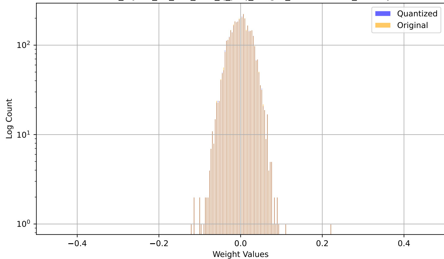
model_layers_31_self_attn_q_proj_weight_channel3185_overlay
