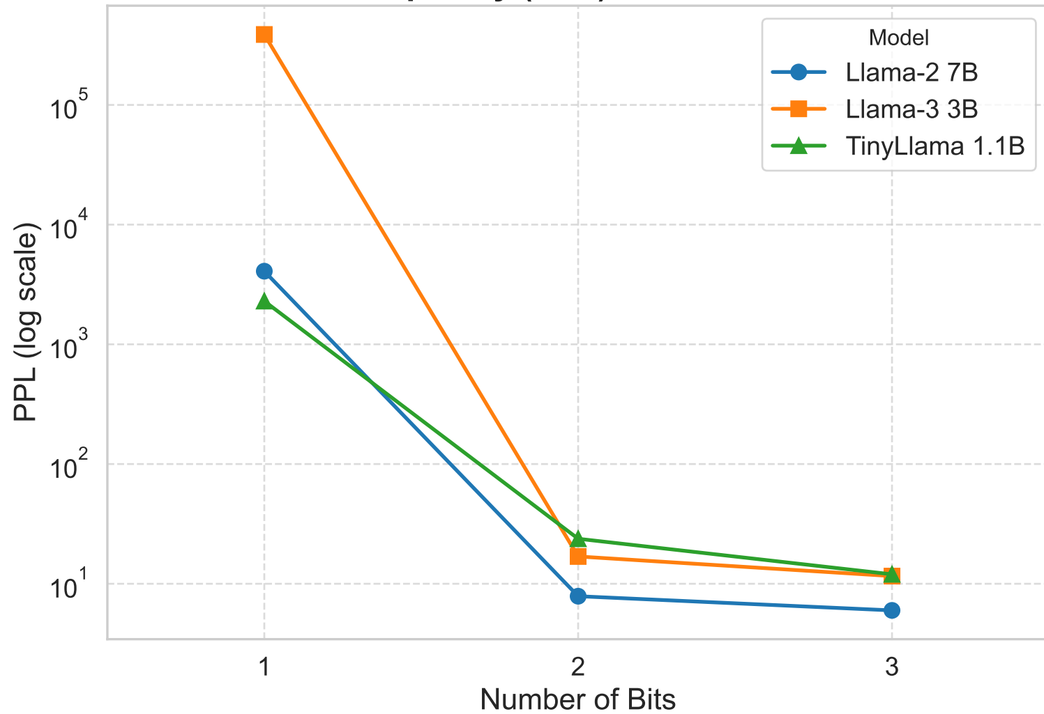
Perplexity (PPL) vs Bit Level
