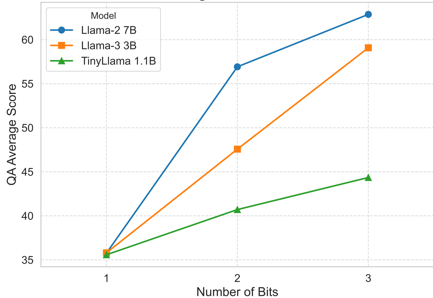
QA Average Score vs Bit Level
