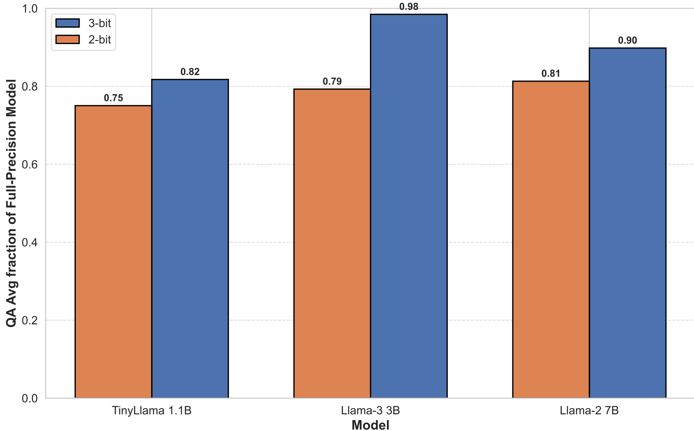
QA Performance vs Full-Precision Model
