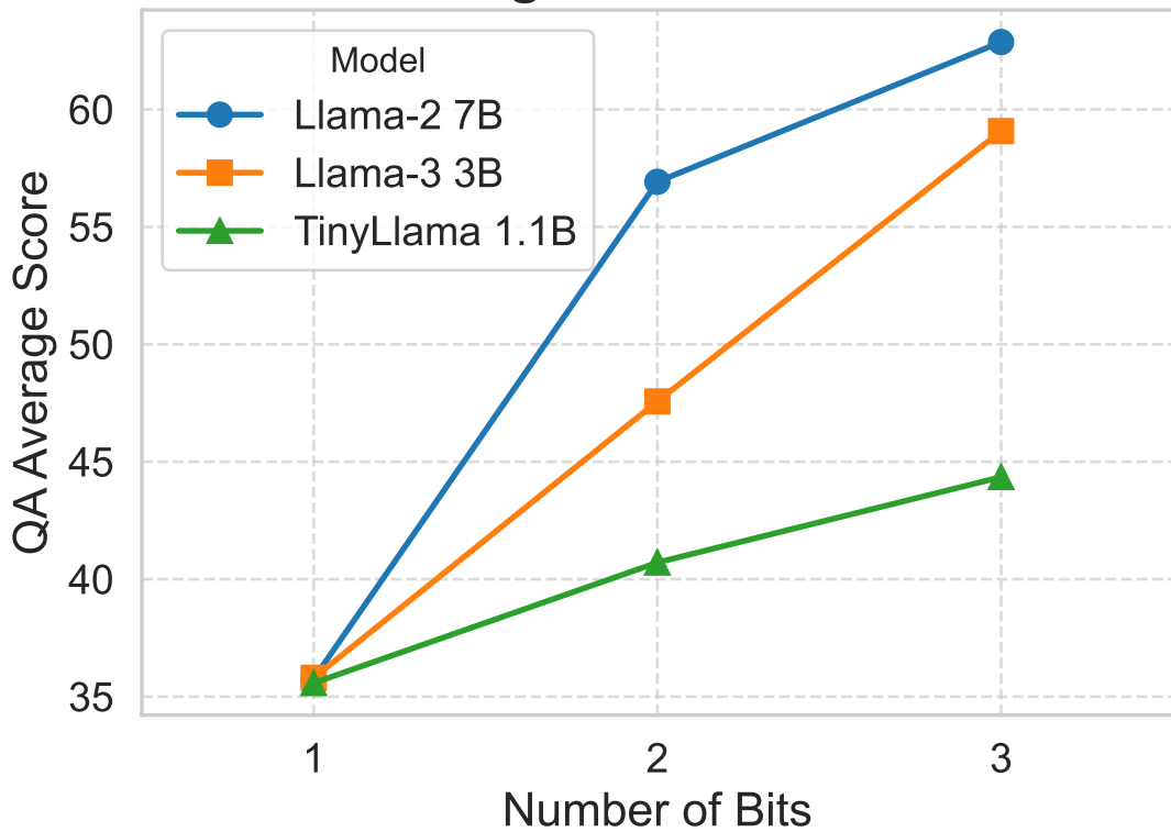
QA Average Score vs Bit Level
