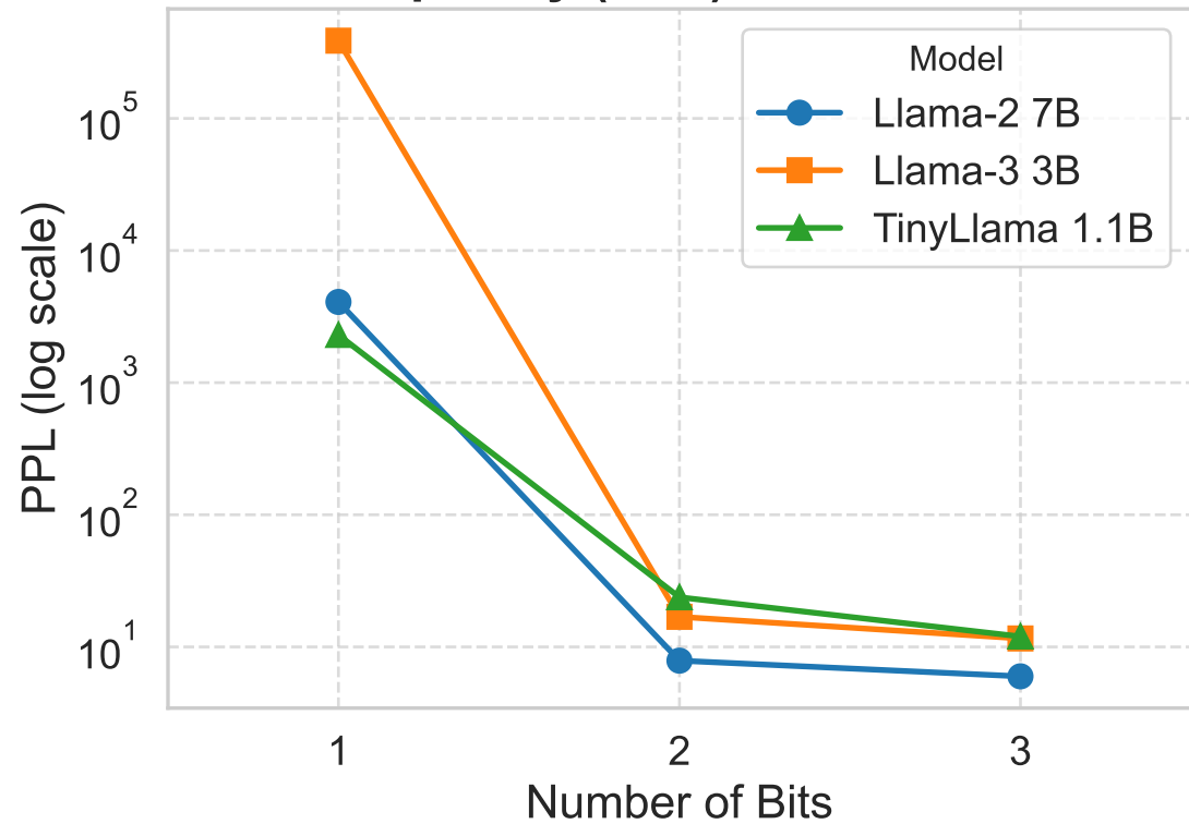
Perplexity (PPL) vs Bit Level
