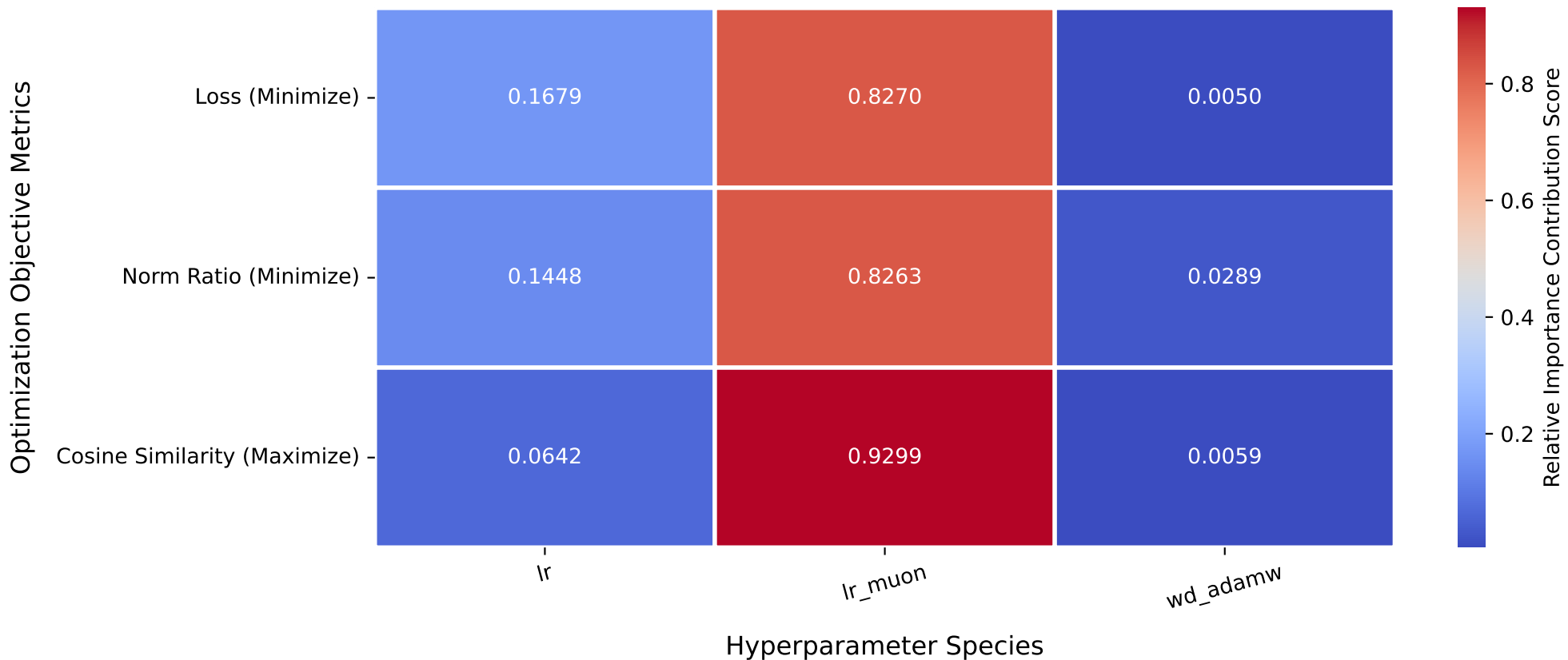
Global Hyperparameter Importance Phase Heatmap
