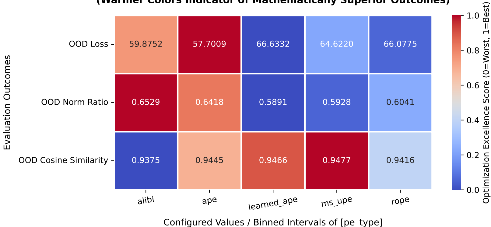
Ablation Analysis Portrait: Parameter [pe_type] (Warmer Colors Indicator of Mathematically Superior Outcomes)
