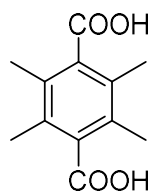
\text{H}_2\text{TMBDC}
