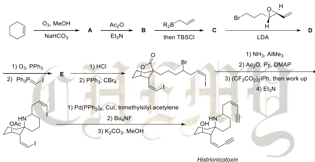
Histrionicotoxin
