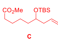
Histrionicotoxin
