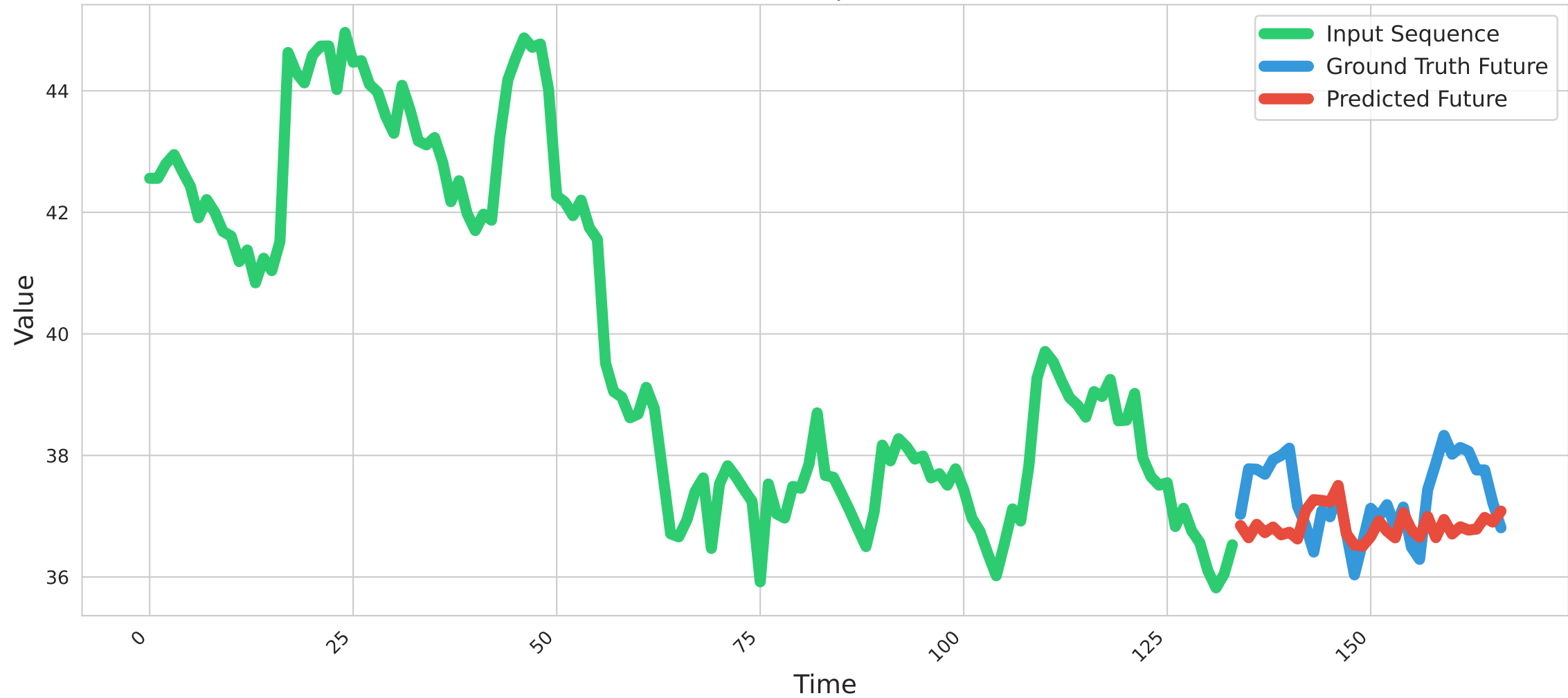
Time Series Prediction Sample MAPE: 1.680604 | MAE: 0.632619
