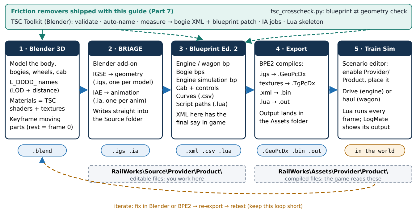
Figure 0.1 · The five stages and what each produces. The teal lane is the tooling from Part 7 that removes the manual copy-paste steps (measuring bogie pivots, re-typing coupling positions, checking node names). Everything left of the Export box lives in Source ; everything the game loads lives in Assets .
