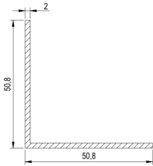
Cantoneira 2" leve
