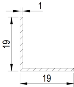
Cantoneira 3/4" leve
