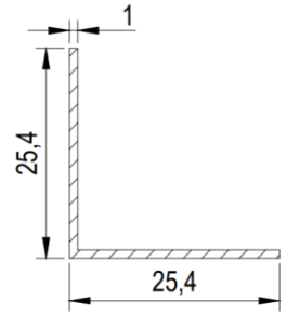
Cantoneira 1" leve
