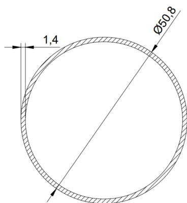
Tubo 2"
