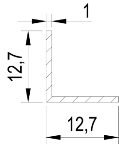
Cantoneira 1/2" leve
