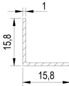
Cantoneira 5/8" leve
