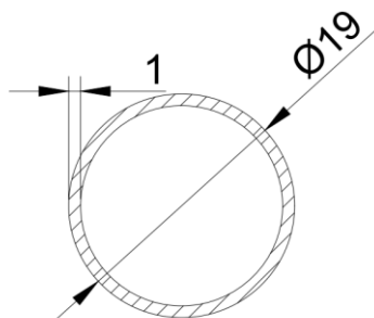
Tubo 3/4"
