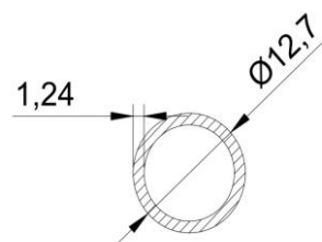
Tubo 1/2"
