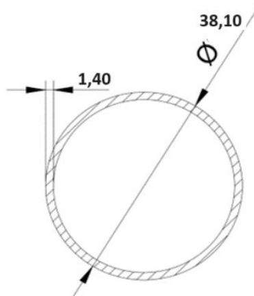
Tubo 1.1/2"
