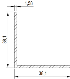
Cantoneira 1.1/2" leve
