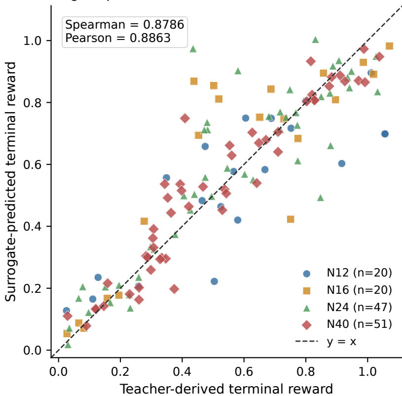
Surrogate-predicted vs teacher-derived terminal reward
