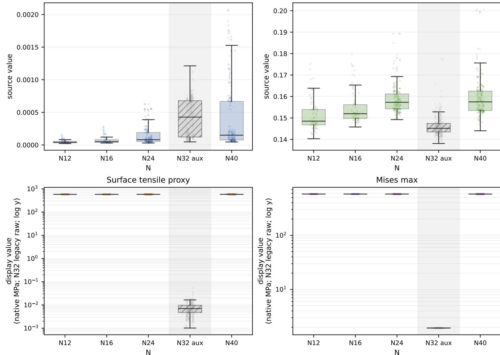
Figure 3.4. Abaqus reward-response metric distributions with auxiliary N32
