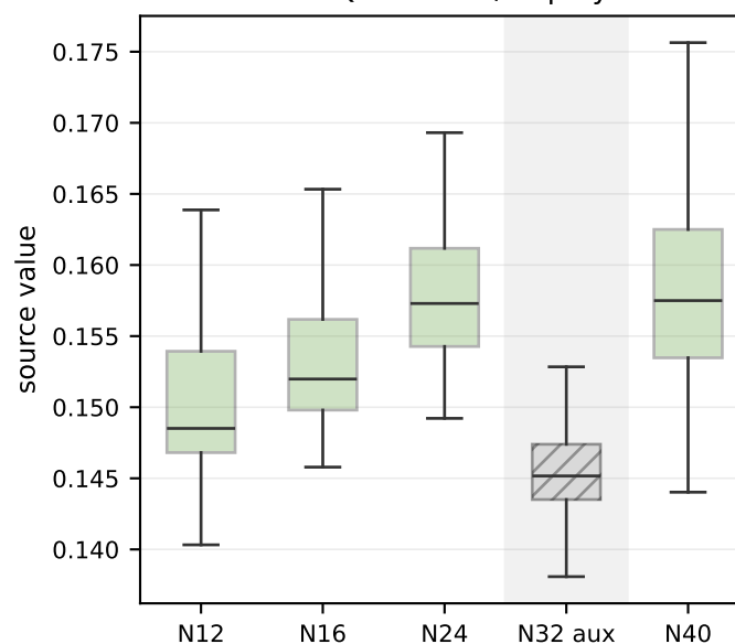
Figure 3.5. Raw/display ranges versus within-N normalization with auxiliary N32
