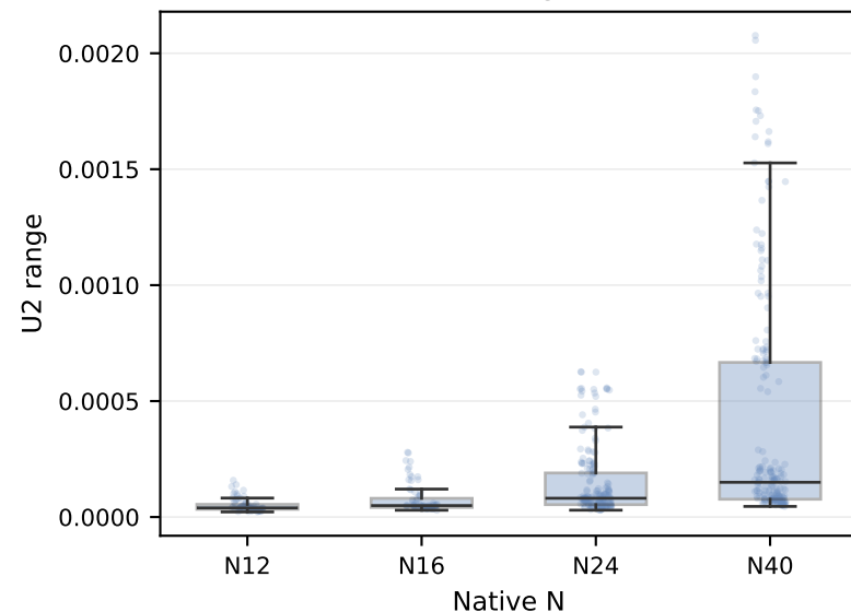
Figure 3.4. Abaqus teacher metric distributions by native N
