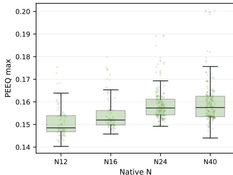
Figure 3.4. Abaqus teacher metric distributions by native N
