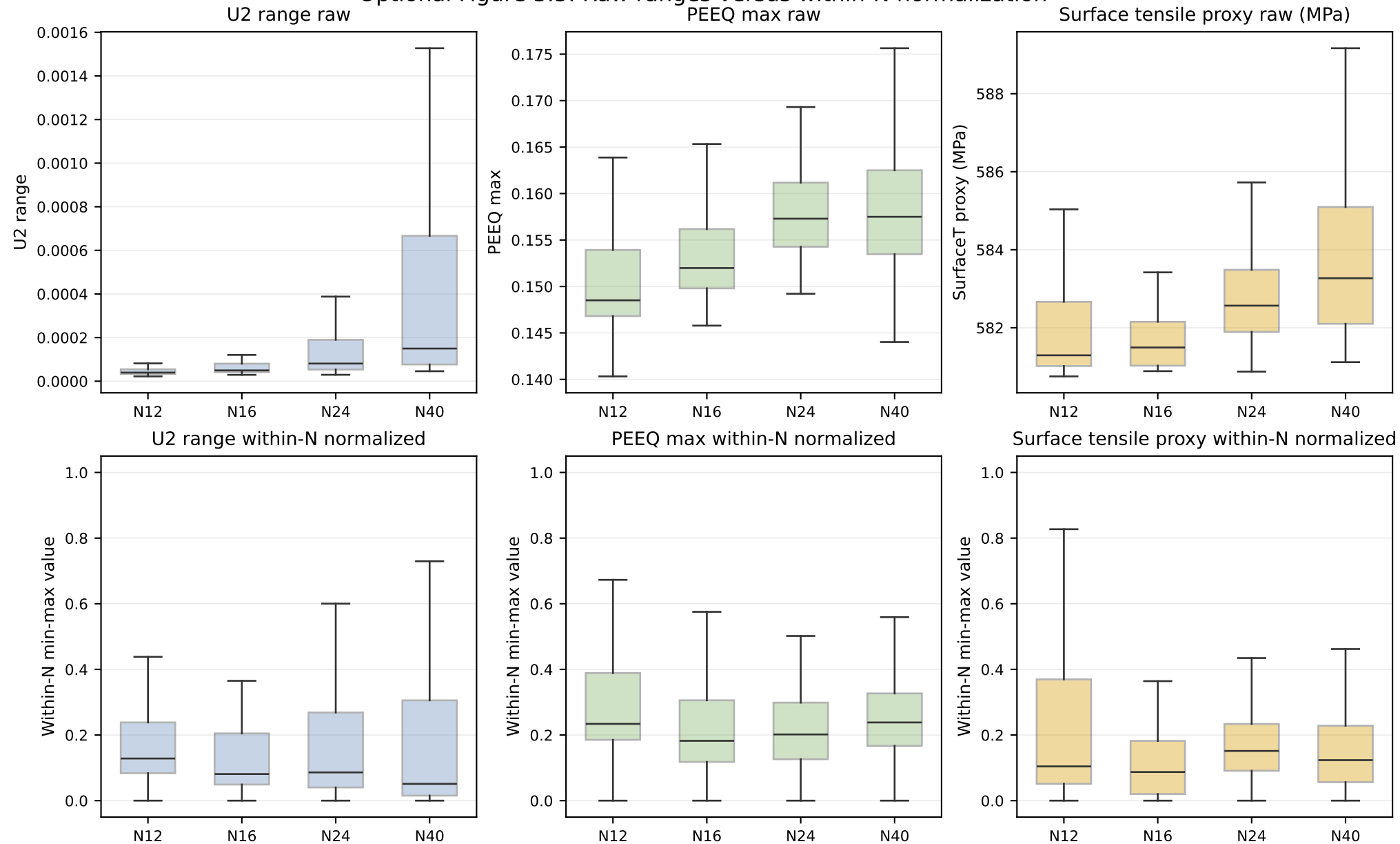
Optional Figure 3.5. Raw ranges versus within-N normalization
