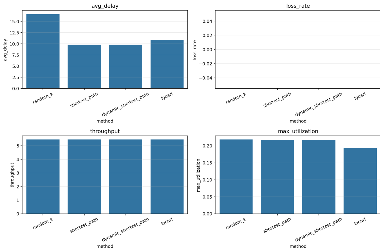
Figure 3. Evaluation bar charts comparing LG-CARL with routing baselines.
