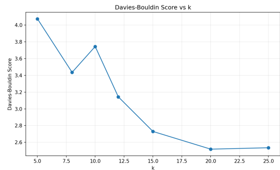
Figure 4: Davies-Bouldin Score vs. K.
