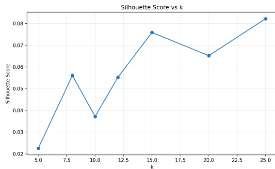
Figure 3: Silhouette Score vs. K.
