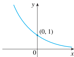
(a) y = a^x , 0 < a < 1
