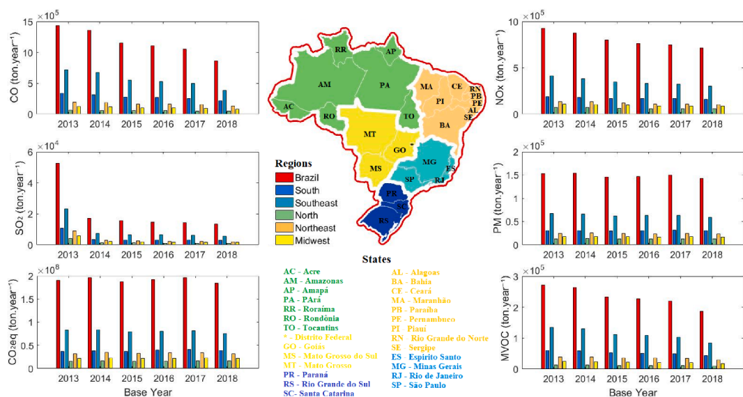
Fig. 1. Vehicular emissions of CO, SO 2 , CO 2 eq, NO x , PM, and NMVOC in Brazil from 2013 and 2018 estimated by BRAVES using emission factors from CETESB.
