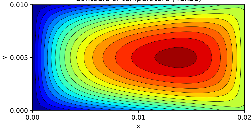
Contours of temperature (41x21)
