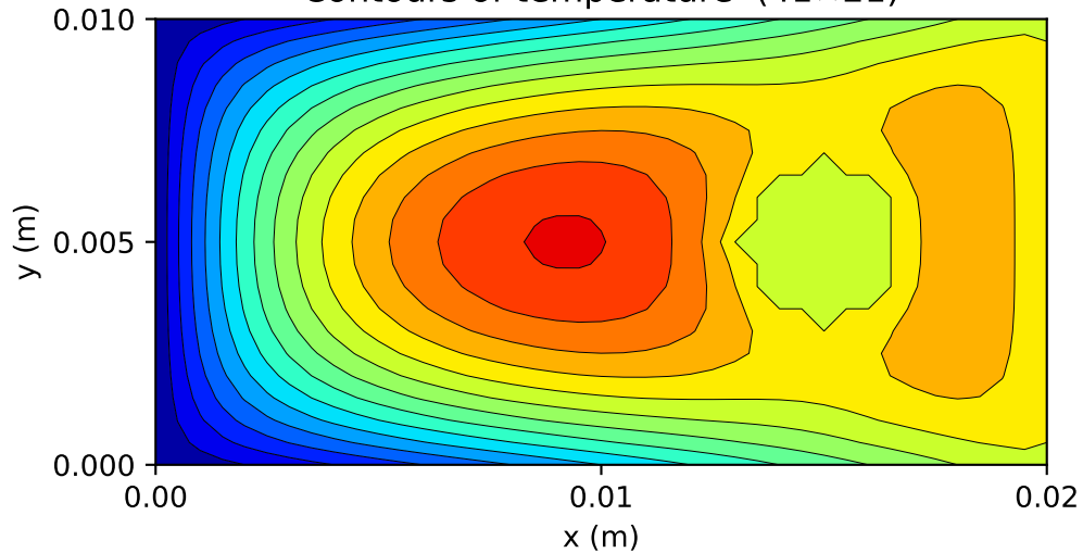
Contours of temperature (41×21)
