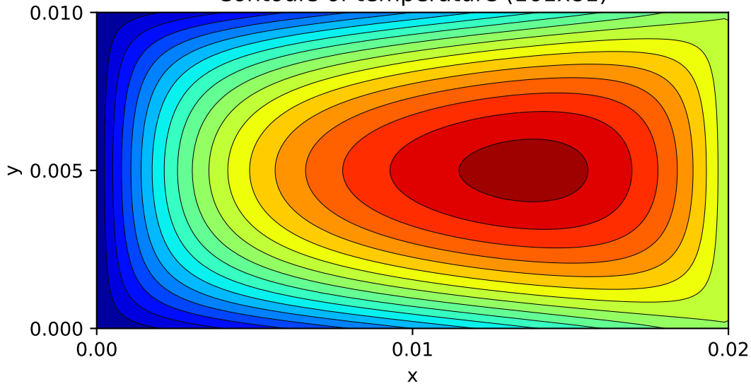
Contours of temperature (161x81)
