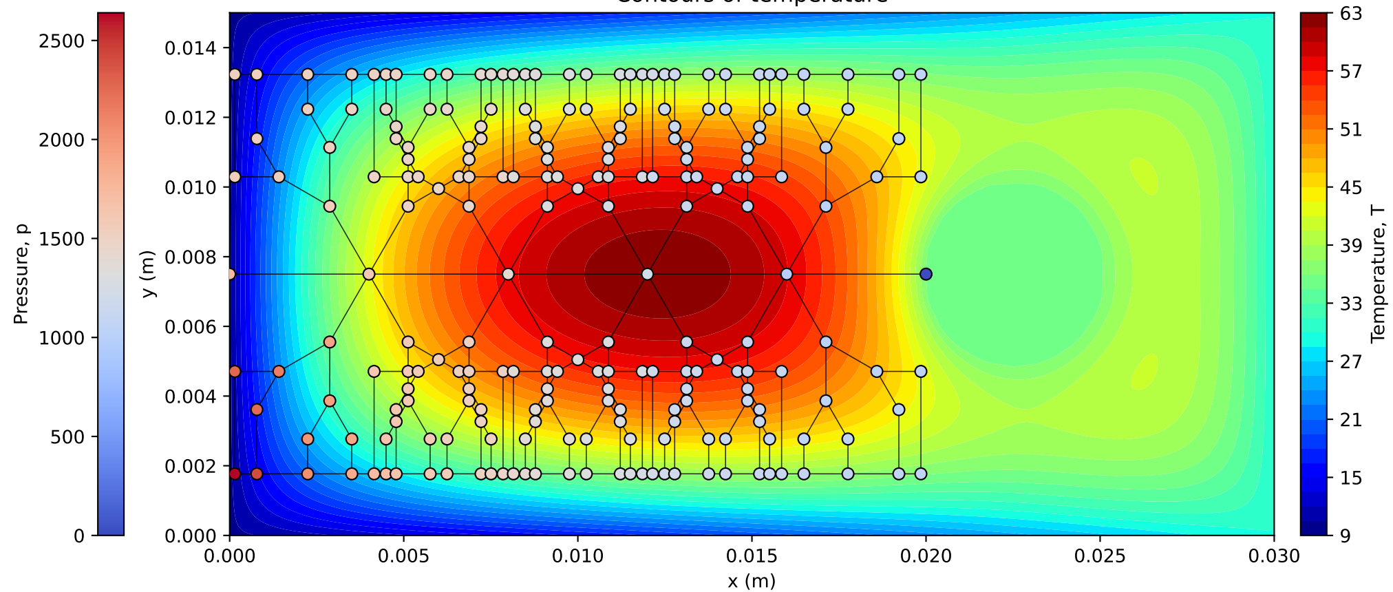
Contours of temperature
