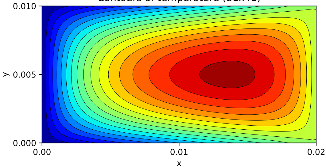
Contours of temperature (81x41)
