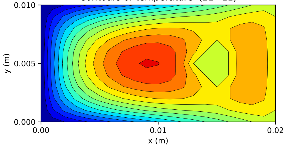
Contours of temperature (21×11)
