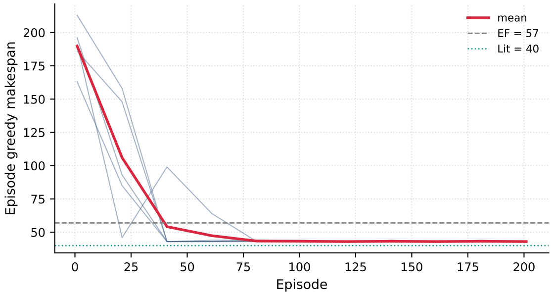
Per-action REINFORCE on MK01 (5 seeds, 200 ep)
