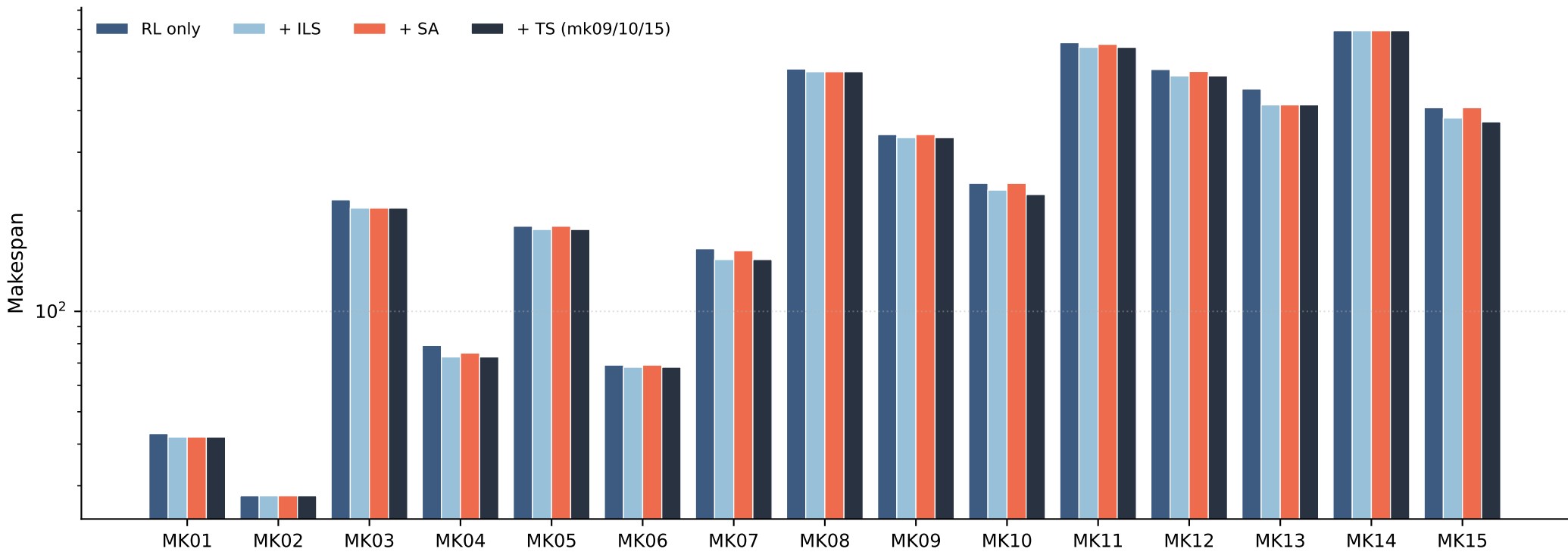
Per-instance ablation: contribution of ILS, SA, TS to the pipeline
