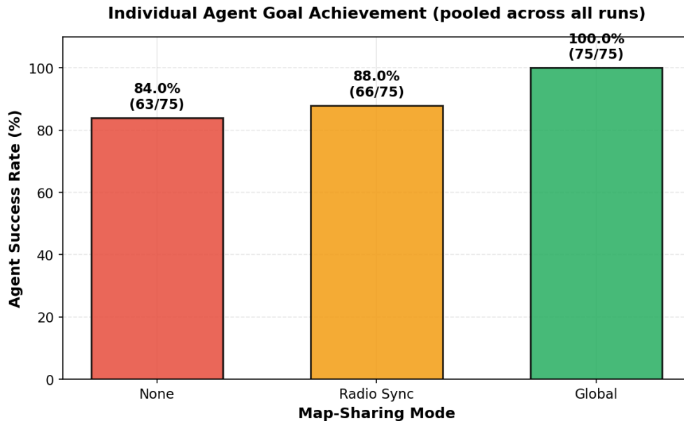
Figure 4: Impact of Map Sharing on Task Completion. Global sharing guarantees success, while Radio synchronization fails to maintain connectivity sufficient to outperform the baseline significantly.
