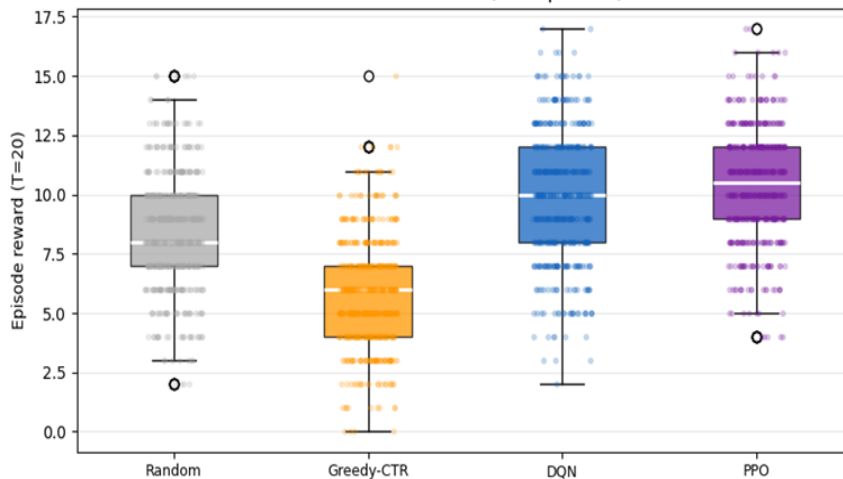
Reward Distribution (500 episodes)
