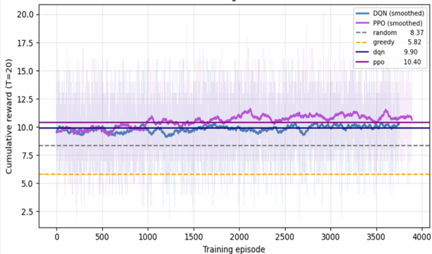
Learning Curves
