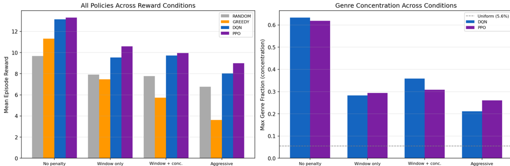
Reward Shaping Experiment Summary
