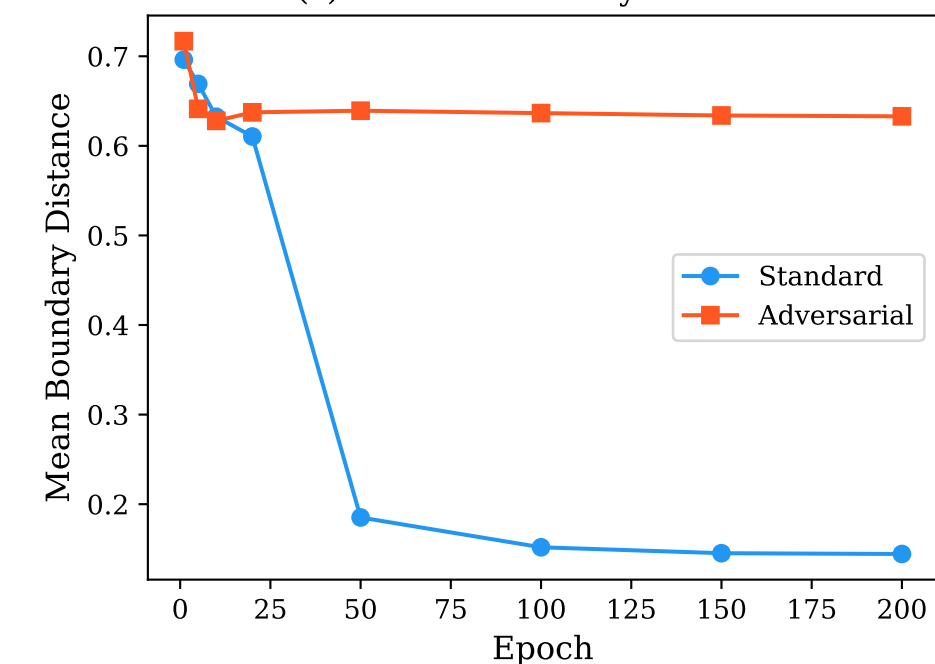
(c) Data-to-Boundary Distance
