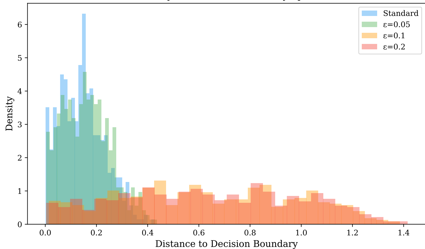
Boundary Distance Distribution by Epsilon
