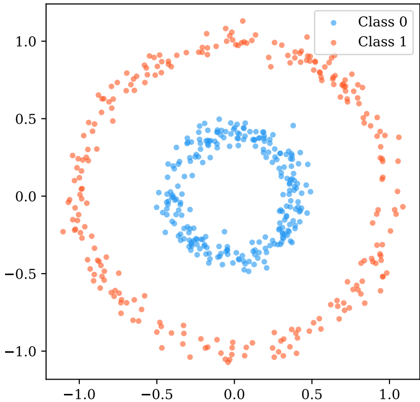
Dataset: concentric_rings
