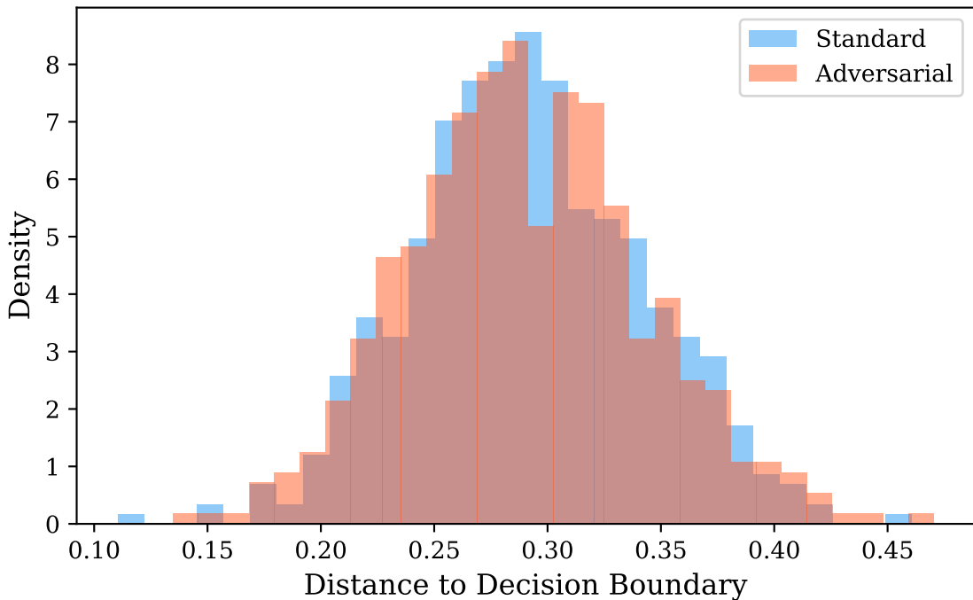
Boundary Distance Distribution (Epoch 200)
