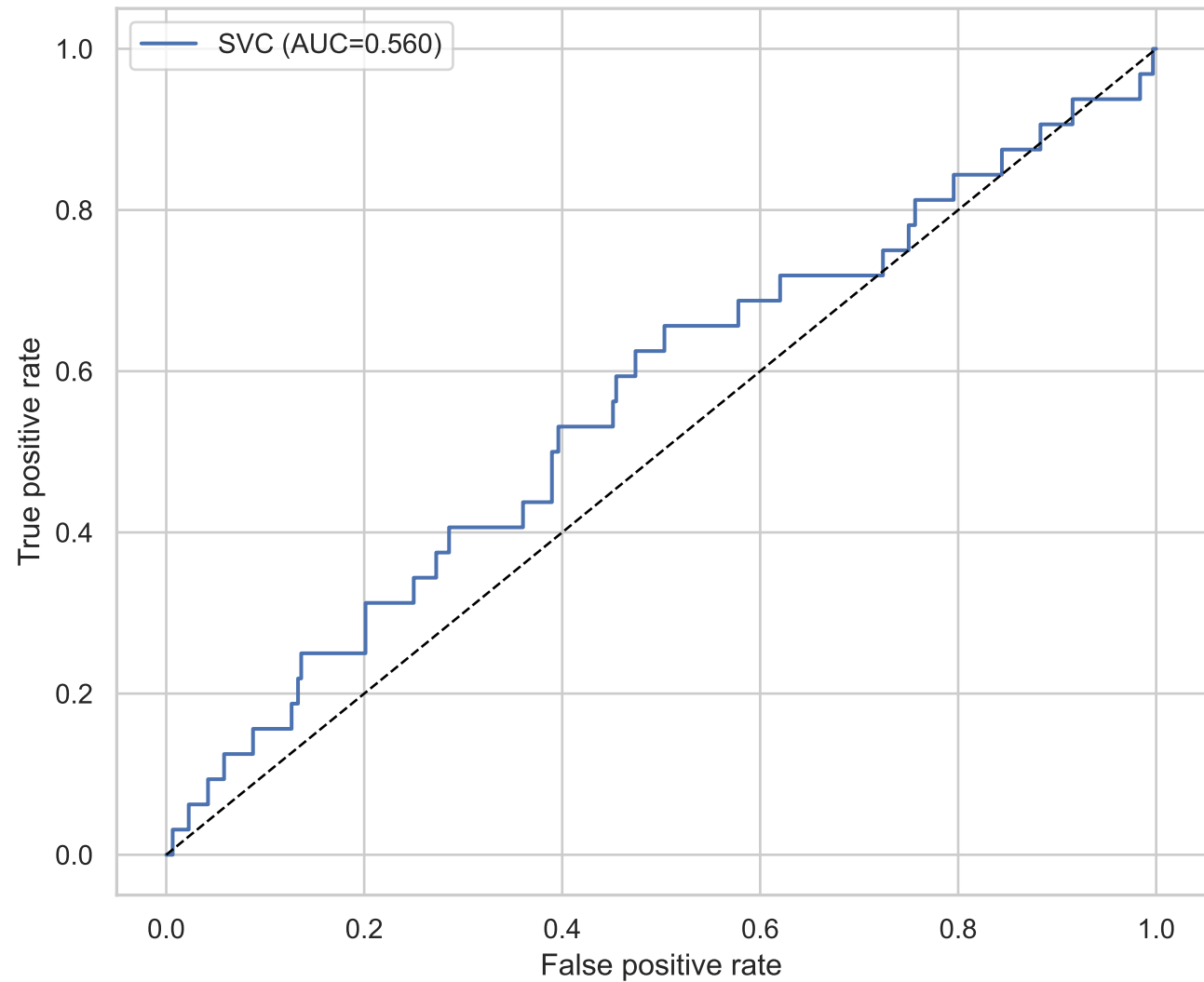
Final model ROC curve on the held-out test set
