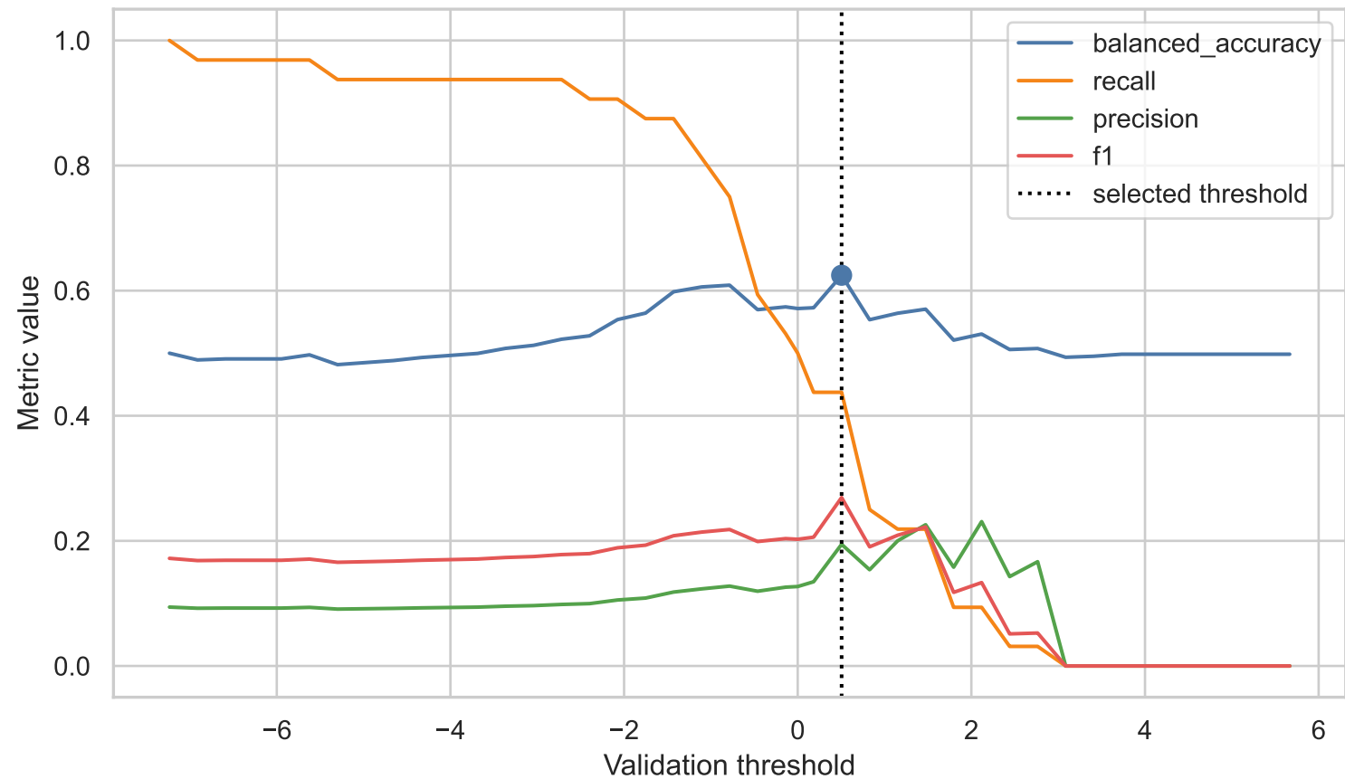
Validation threshold trade-offs for SVC
