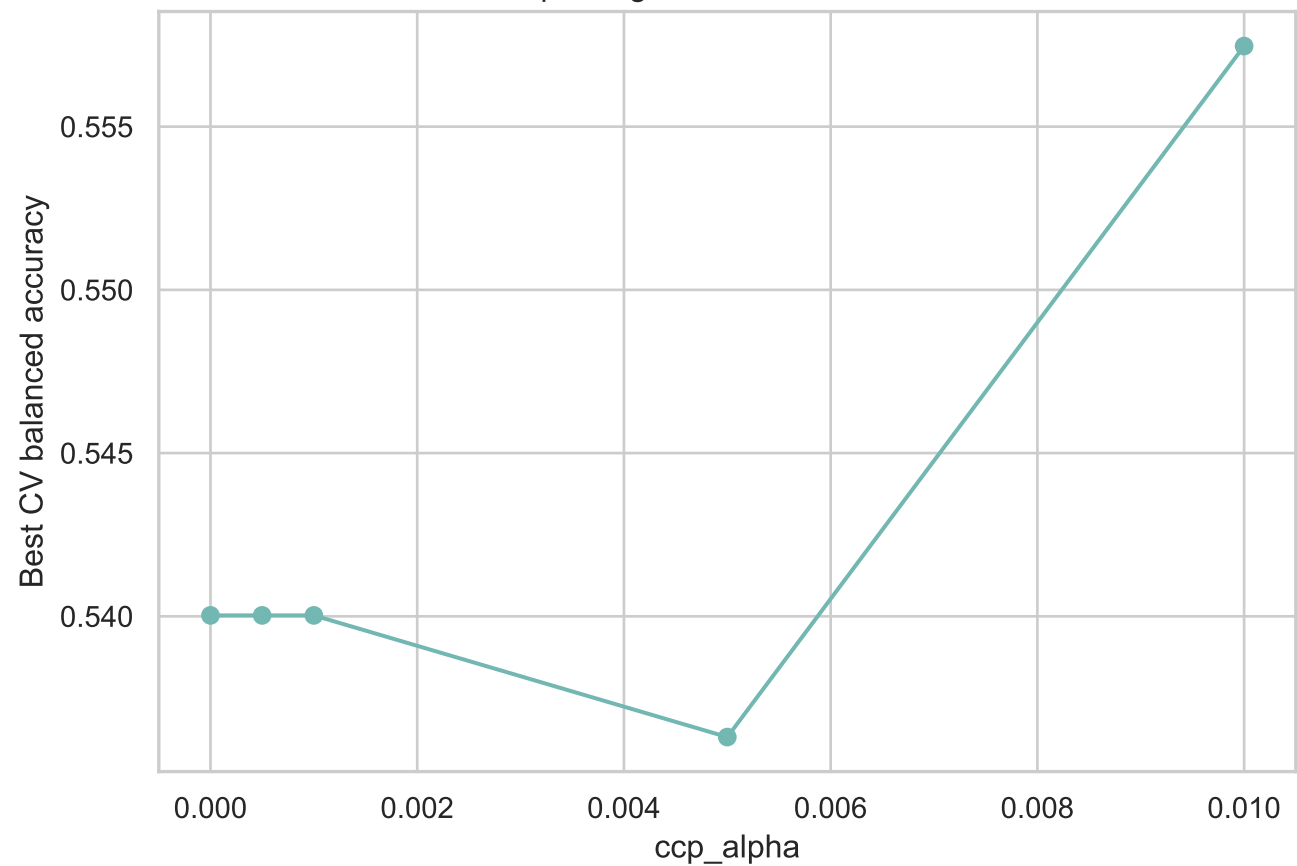
Decision-tree pruning curve from manual fold-local CV
