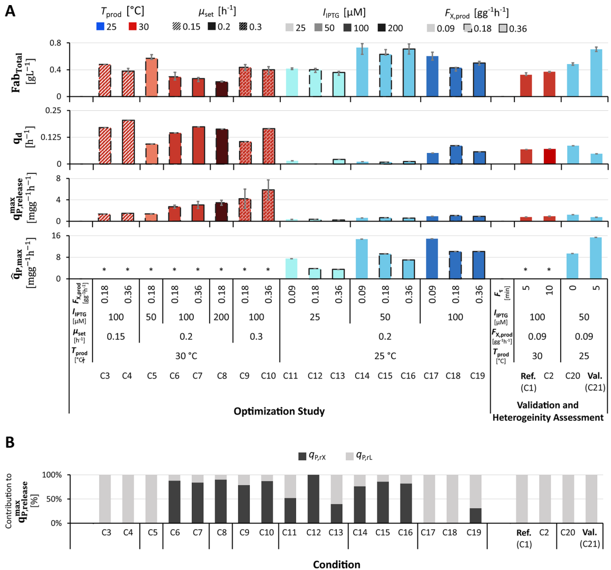
Fig. 5 Screening results of an E. coli -based Fab antibody production process with product release, evaluated using the optimization targets total Fab titer ( \text{Fab}_{\text{Total}} ), cell lysis rate ( q_{\text{d}} ), maximum specific product release rate ( q_{\text{P,release}} ), and maximum specific product formation rate ( q_{\text{P}} ). (A) Results obtained for 20 process conditions, including the starting condition (reference, Ref.), and compared with an independent validation experiment (Val.). The figure further indicates which conditions were used to investigate substrate heterogeneities through different feeding regimes ( F_{\text{T}} ) and which were included exclusively for process optimization. Process conditions are encoded by the post-
