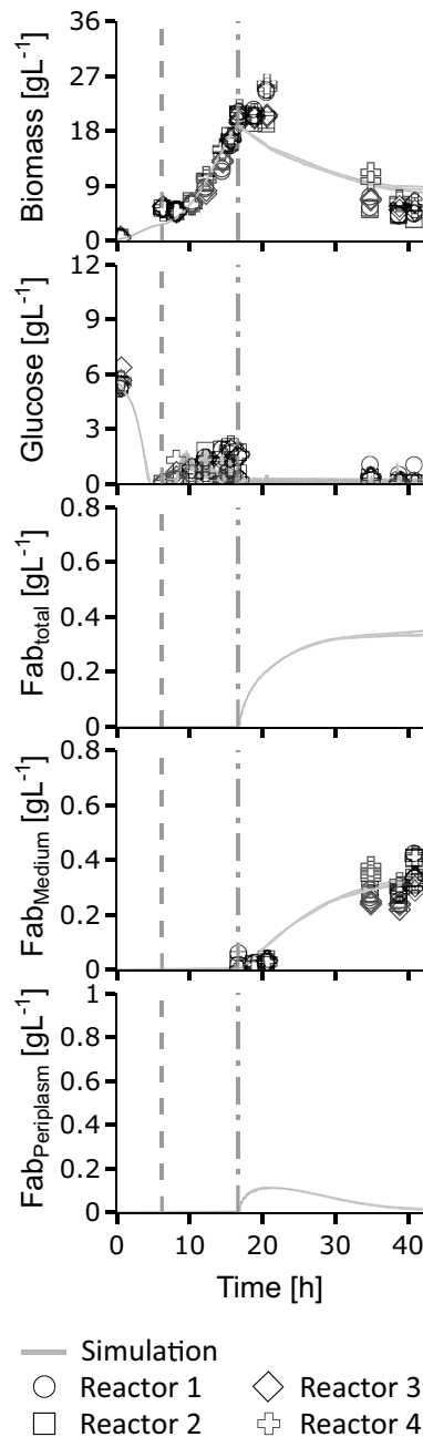
Fig. 1 E. coli K-12 fed-batch cultivation with Fab production and release under reference conditions. Experimental data (open markers) and predictions of the mechanistic model (solid lines) from Schröder-Kleeberg et al. [25] are shown. The gray vertical dashed and dot-dashed lines indicate the start of feeding and the time of induction, respectively
