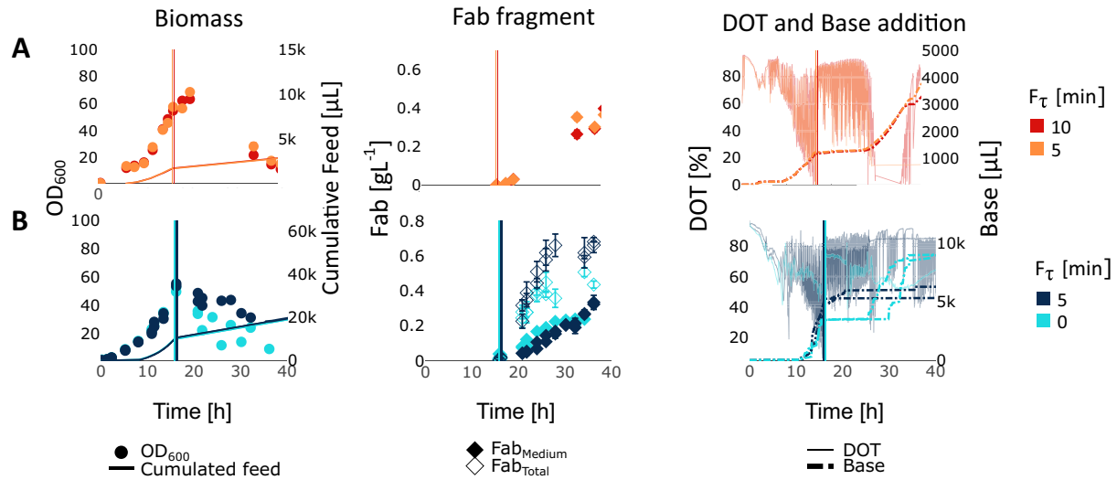
Fig. 4 Process data from validation experiments and investigations of robustness against heterogeneous substrate conditions. Applied experimental conditions are given as T_{\text{prod}}/\mu_{\text{set}}/F_{X,\text{prod}}/I_{\text{IPTG}}/F_{\tau} , corresponding to production temperature ( ^{\circ}\text{C} ), specific pre-induction growth rate ( \text{h}^{-1} ), specific post-induction feed rate ( \text{g g}^{-1} \text{h}^{-1} ), induction strength with IPTG ( \mu\text{M} ), and heterogeneous substrate conditions (min), respectively. Variable process conditions are indicated by an “x” (e.g., x/\mu_{\text{set}}/F_{X,\text{prod}}/I_{\text{IPTG}}/F_{\tau} ). A The effect of increased substrate heterogeneity was investigated using larger pulse-based feeding intervals at 15 mL scale (30/stepwise feeding/0.09/100/x)
