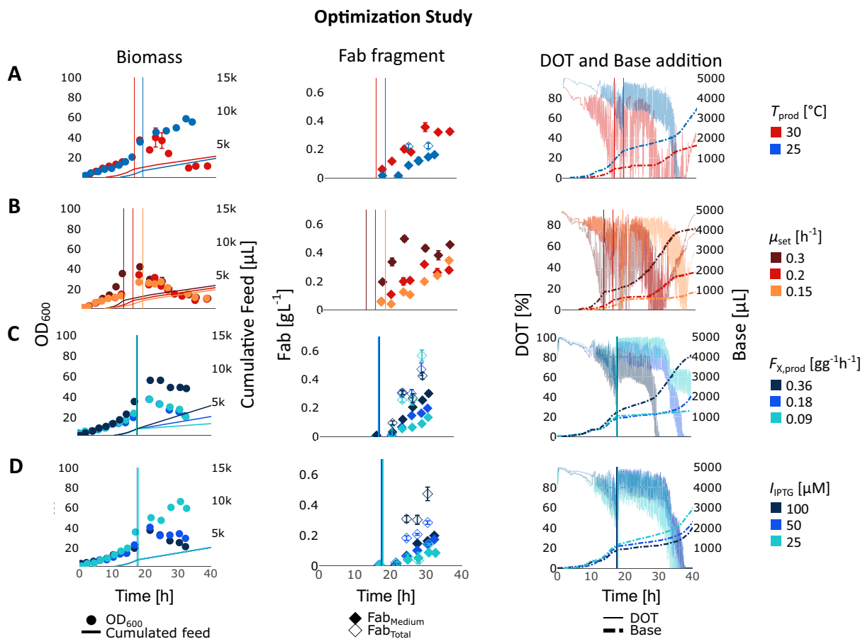
Fig. 2 Selected process data from the optimization study. Applied experimental conditions are given as T_{prod}/\mu_{set}/F_{X,prod}/I_{IPTG}/F_T , corresponding to production temperature ( ^{\circ}\text{C} ), specific pre-induction growth rate ( \text{h}^{-1} ), specific post-induction feed rate ( \text{gg}^{-1}\text{h}^{-1} ), induction strength with IPTG ( \mu\text{M} ), and heterogeneous substrate conditions (min), respectively. Varying conditions are indicated by an “x” (e.g., x/\mu_{set}/F_{X,prod}/I_{IPTG}/F_T ). Shown are the effects of A production temperature (reference condition vs. 25/0.2/0.18/50/5), B specific
