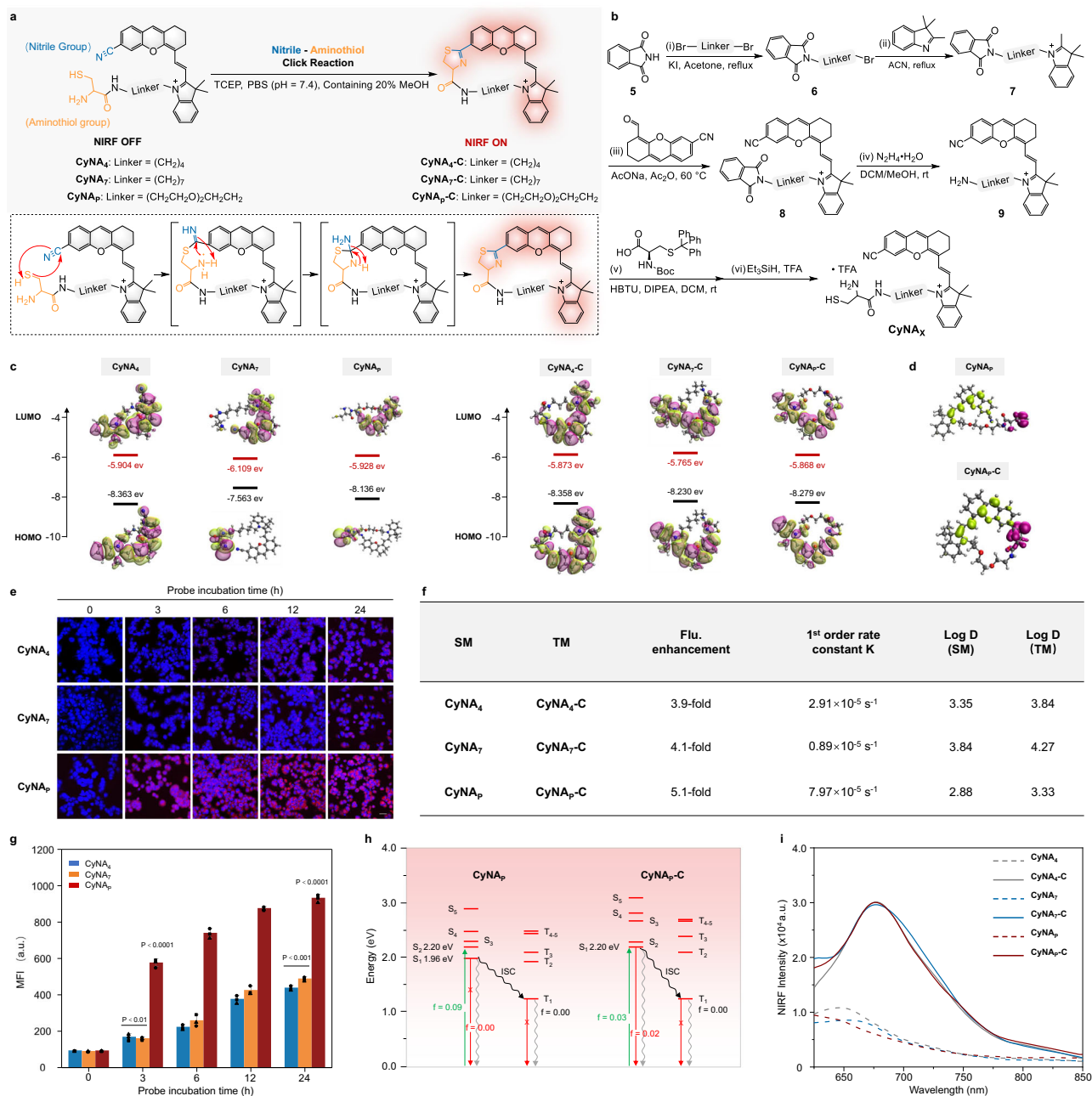
Fig. 3 | Synthesis and screening of CyNA x for intramolecular cyclization.
