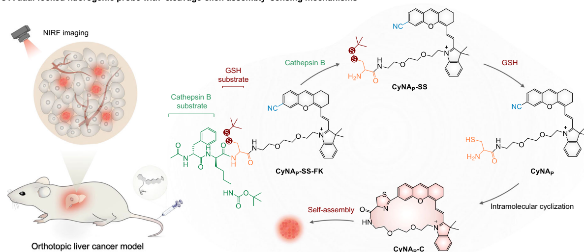
Fig. 1 | Design of NAT bioorthogonal NIR fluorogenic probes. a, b Schematic of CBT-Cys click reaction and NAT click reaction based fluorogenic hemicyanine in this study. c, d Schematic illustration of the intramolecular cyclization and self-assembly mediated by CBT-Cys click reaction c and NAT click reaction d , the
