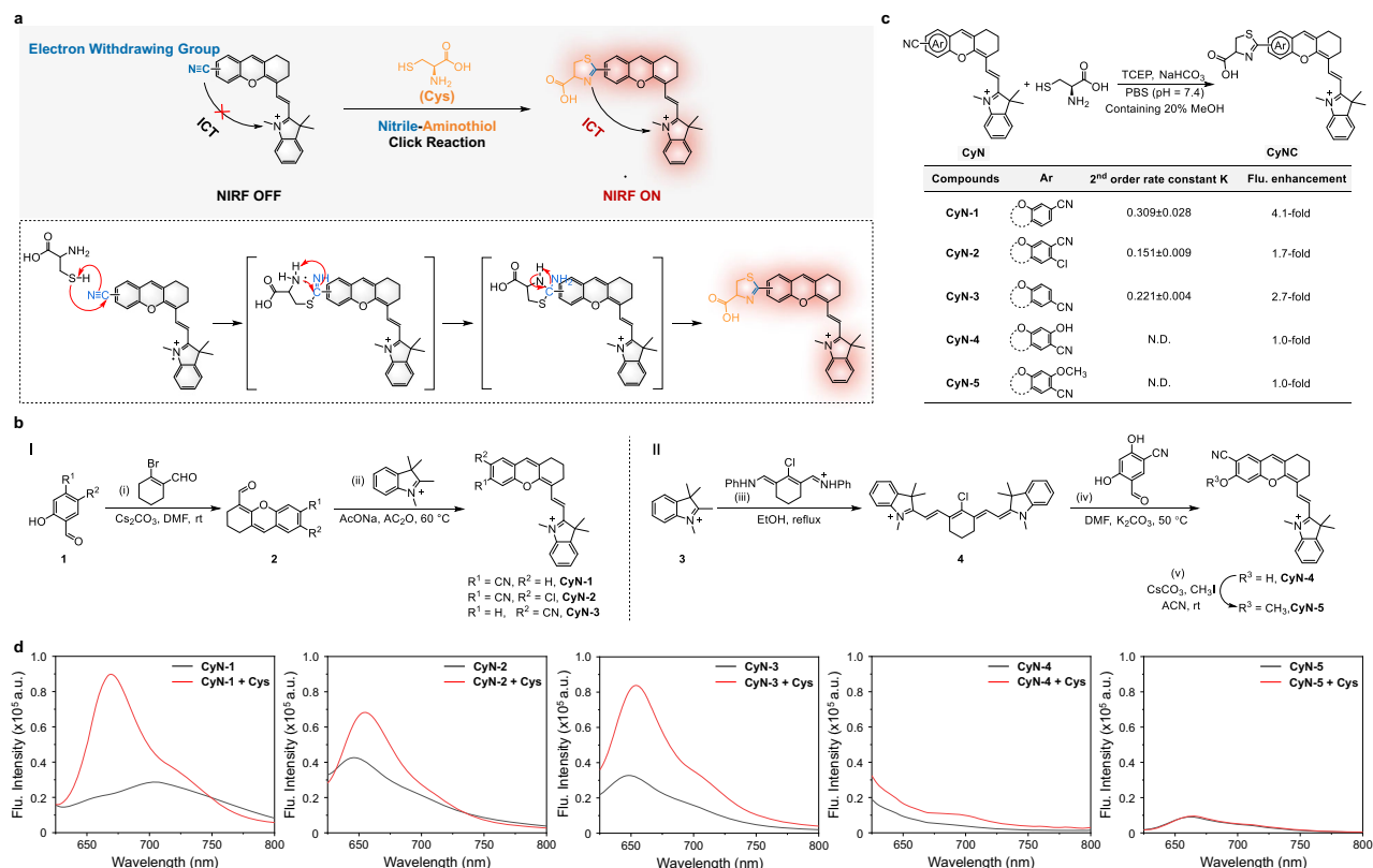
Fig. 2 | Synthesis and screening of NAT bioorthogonal fluorogenic lumino-phores. a Chemical structures and sensing mechanisms of nitrile-substituted hemicyanines with free cysteine via NAT click reaction. b Synthetic routes for CyN-1–5 . Reagents and conditions: (i) 2-bromocyclohex-1-ene-1-carbaldehyde, \text{Cs}_2\text{CO}_3 , DMF, rt, 12 h. (ii) 1,2,3,3-tetramethyl-3H-indolium iodide, AcONa, \text{Ac}_2\text{O} , 60 °C, 2–4 h. (iii) vilsmeier haack reagent, EtOH, reflux, 4 h. (iv) 5-formyl-2,4-dihydroxybenzonitrile, \text{K}_2\text{CO}_3 , DMF, 50 °C, 12 h. (v) \text{Cs}_2\text{CO}_3 , \text{CH}_3\text{I} , ACN, rt, overnight. c The
