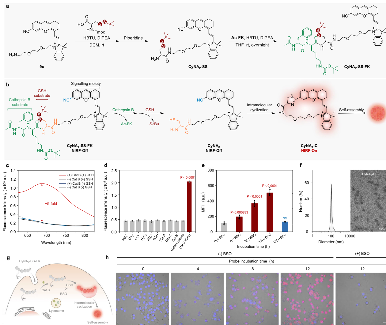
Fig. 5 | Design and characterization of dual-locked fluorogenic probes. a The synthesis route of CyNAp-SS-FK . b Activation mechanism of the dual-locked molecular probe CyNAp-SS-FK for LM3 cell detection. c Fluorescence spectra of CyNAp-SS-FK (20 \mu M) after incubation with/without GSH, Cat B, or GSH and Cat B at 37 ^{\circ} C in PBS buffer (pH 7.4). Fluorescence excitation at 580 nm. d Fluorescence intensity of CyNAp-SS-FK (40 \mu M) after incubation with the indicated enzymes, metal ions (60 \mu M), ROS (60 \mu M) in PBS (10 mM, pH 7.4) at 37 ^{\circ} C. \text{Mg}^{2+} , magnesium chloride; \text{Ca}^{2+} , calcium chloride; \text{ClO}^{-} , sodium hypochlorite; \text{H}_2\text{O}_2 , hydrogen peroxide; \text{SO}_4^{2-} , sodium sulfate; GSH, glutathione; TCEP, Tris(2-carboxyethyl) phosphine hydrochloride; Cas-3, caspase 3; Galactosidase; Cat B, Cathepsin B. ( n = 3 , mean \pm s.d.). Two-tailed Student's t test; GSH and Cat B treated group versus other groups. NS, no statistically significant differences. e Mean NIRF intensities of HCC
