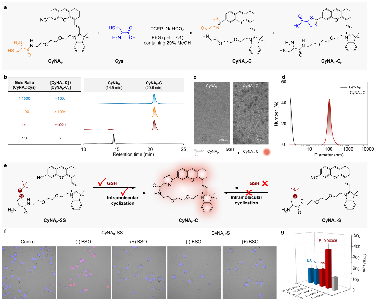
Fig. 4 | ‘Click-Assembly’ and specificity of intramolecular condensation.
