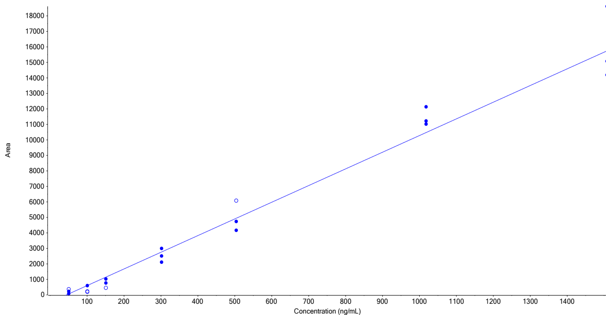
Figure S1: Calibration Curve of 60-mer RNA: To perform absolute quantification an external calibration curve with the 60-mer RNA construct was prepared between 50 – 1500 ng/mL and measured n = 3 . The assay was validated using ICH m10 bioanalytical method development guidance.
