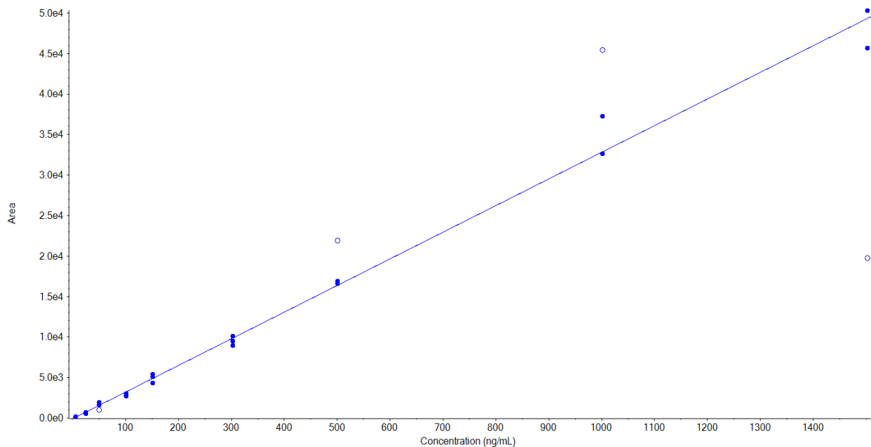
Figure S2: Calibration Curve of Antisense FLuc-S1 dsRNA construct: To perform absolute quantification an external calibration curve with the FLuc-S1 RNA construct was prepared between 5 – 1500 ng/mL and measured n = 3 . The assay was validated using ICH m10 bioanalytical method development guidance.
