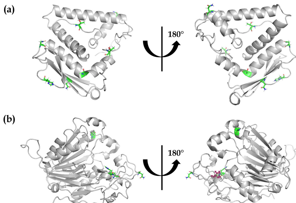
FIGURE 7 | Structural analysis of the N-terminal and C-terminal peptides of CHO PLBL2 using a homology model predicted by AlphaFold2 using UniProt entry G3I6T1 (with the signaling sequences removed). Shown in color are residues which exhibit post-translational modifications (including N-linked glycosylation, O-linked glycosylation, and phosphorylation). (a) Front and back views of the N-terminal peptide. (b) Front and back views of the C-terminal peptide.
