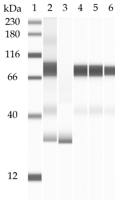
FIGURE 3 | Affinity capture of CHO PLBL2 from pembrolizumab and subsequent enrichment, as detected via capillary Western blot. Lane 1: molecular weight marker. Lane 2: pembrolizumab starting material (pre-enrichment, “load”), which exhibits multiple molecular weight isoforms (~80 kDa, ~45 kDa, and ~30 kDa) of endogenous CHO PLBL2. Lane 3: pembrolizumab after affinity capture (“depleted”), which exhibits depletion of the ~80 kDa and ~45 kDa isoforms of endogenous CHO PLBL2 but retention of the ~30 kDa isoform. Lanes 4–6: enriched fractions, which exhibit recovery and enrichment of primarily the ~80 kDa and ~45 kDa isoforms of endogenous CHO PLBL2.
