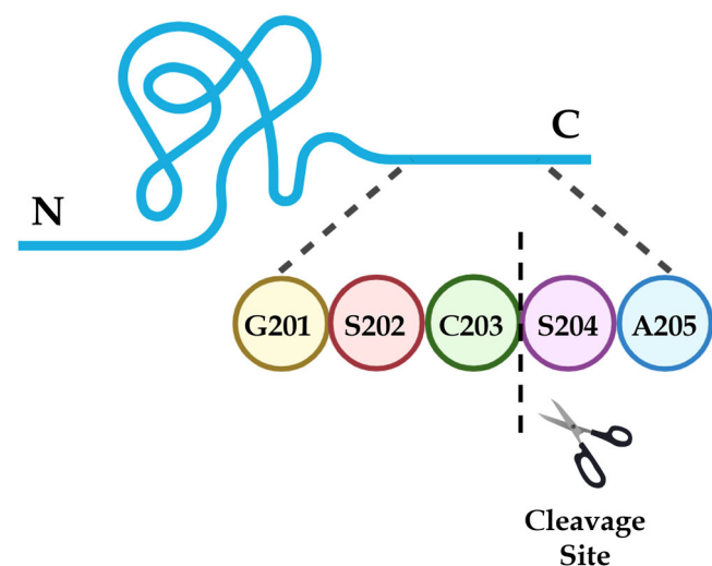
FIGURE 4 | Cleavage site between C203 and S204, identified by peptide mapping in CHO PLBL2 captured from pembrolizumab. Truncation at this site yields an N-terminal peptide of approximately 28 kDa and a C-terminal peptide of approximately 44 kDa.
