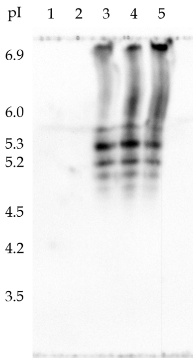
FIGURE 2 | Analysis via IEF gel and Western blot of the charge variants of CHO PLBL2 captured from pembrolizumab. Lanes 1–2: isoelectric point (pI) markers. Lanes 3–5: enriched CHO PLBL2. Numerous distinct protein bands are observed between pIs of about 5.0 and about 6.0, indicating a diverse array of charge isoforms for CHO PLBL2 within this range. Bands are also observed at pIs > 6.9, which were not fully resolved. For reference, the theoretical pI for CHO PLBL2 (calculated based on the amino acid sequence of UniProt entry G3I6T1) is 5.63.
