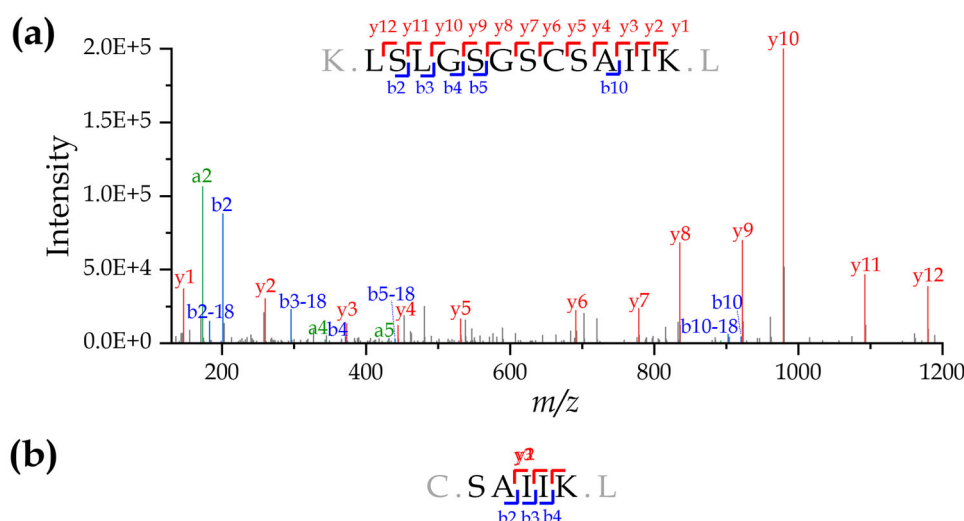
FIGURE 5 | Tandem mass spectrum sequencing evidence confirming the cleavage site between C203 and S204 in CHO PLBL2 captured from pembrolizumab. Peptide mapping analysis generated high-quality tandem mass spectra for (a) the full-length tryptic peptide LSLGSGSC*SAIK and (b) the C-terminal tryptic peptide SAIK , which resulted from C203/S204 cleavage. Note: As described in the Materials and Methods, cysteine was alkylated with iodoacetamide, resulting in carbamidomethylation (+57 Da).
