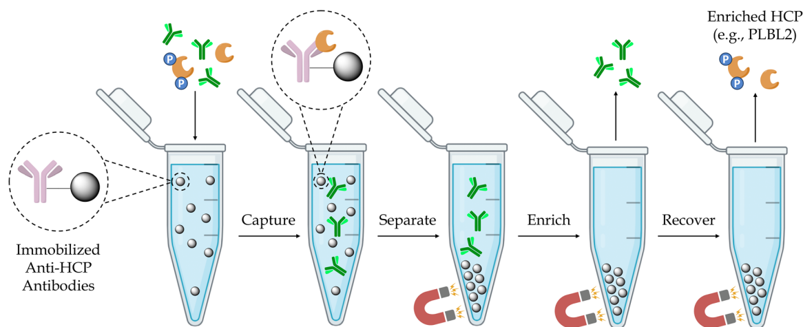
SCHEME 1 | Affinity capture of a target host cell protein and its various proteoforms (e.g., CHO PLBL2, shown in orange) from a therapeutic antibody (e.g., pembrolizumab, an IgG4) using immobilized polyclonal antibodies directed against the HCP of interest, followed by enrichment and recovery of the target HCP and its proteoforms from the resin for subsequent characterization.
