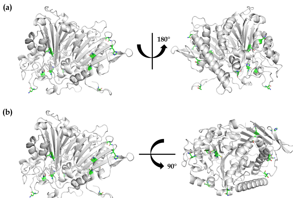
FIGURE 6 | Structural analysis of intact CHO PLBL2 using a homology model predicted by AlphaFold2 using UniProt entry G3I6T1 (with the signaling sequence removed). Shown in color are residues which exhibit post-translational modifications (including N-linked glycosylation, O-linked glycosylation, and phosphorylation) and the cleavage site to render N-terminal and C-terminal peptides. (a) Front and back views of intact CHO PLBL2. (b) Front and top views of intact CHO PLBL2.
