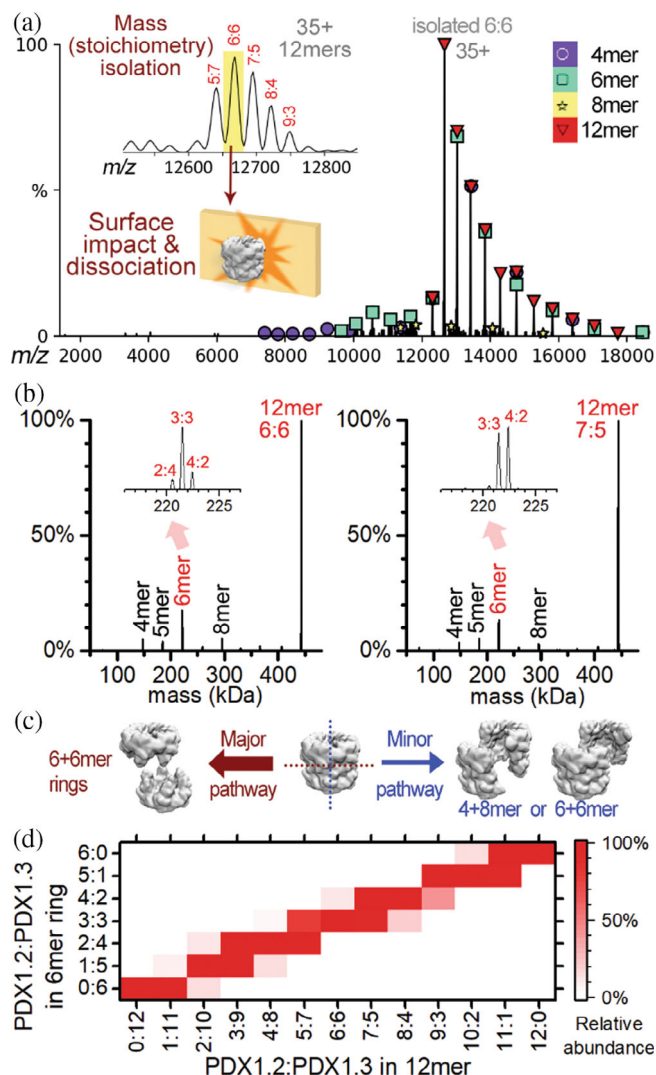
FIGURE 3 Surface-induced dissociation (SID) of pyridoxine biosynthesis enzyme (PDX) 12mers in the gas phase. (a) Representative SID spectrum for a 12mer with a single stoichiometry of 6:6 (PDX1.2/PDX1.3). The 6:6 stoichiometry was isolated and collided with a surface to produce the subcomplexes shown in the mass spectrum, each labeled by symbols indicated on the top right. (b) Deconvoluted mass distribution of SID spectra for 6:6 (left) and 7:5 (right), with zoomed-in views of the 6mer region shown as insets. (c) Proposed dissociation pathways leading to different subcomplexes, with the major pathway splitting the 12mer into 6mers. (d) Heat map displaying the normalized relative abundance of released 6mer rings from major pathway (vertical axis) from each stoichiometry of 12mers (horizontal axis). The stoichiometry of the released 6mer is almost exclusively half of the 12mer precursor, suggesting that the assembly is not completely random and has degrees of symmetry. Reprinted with permission from Novikova et al. (2021). Copyright 2021 American Chemical Society.
