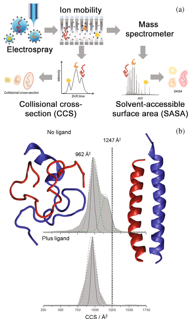
FIGURE 4 (a) Schematic of ESI-IM-MS analysis and the resulting structural parameters. (b) CCS distributions derived from arrival time distributions for the [M + 5H]^{5+} ions of c-MYC-Zip: MAX-Zip. Results in the absence of ligand and in the presence of ligand are shown in the top and bottom panels, respectively. In the absence of ligand, the complexes exist in two conformations, one extended and one compact (top panel). The presence of ligand inhibits ordered complex formation (bottom panel). Profiles for the predicted conformation from simulated annealing (solid lines) and from NMR structures (vertical dotted line) are displayed together with experimental fitted curves (dashed lines). Adapted with permissions from Santambrogio et al. (2022). Copyright 2022 Elsevier B.V., and Harvey et al. (2012). Copyright 2012 American Chemical Society.
