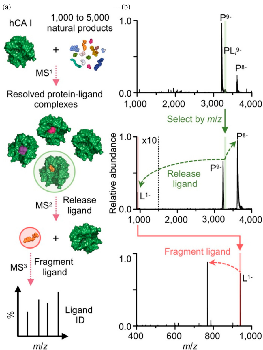
FIGURE 2 Multistage tandem MS
