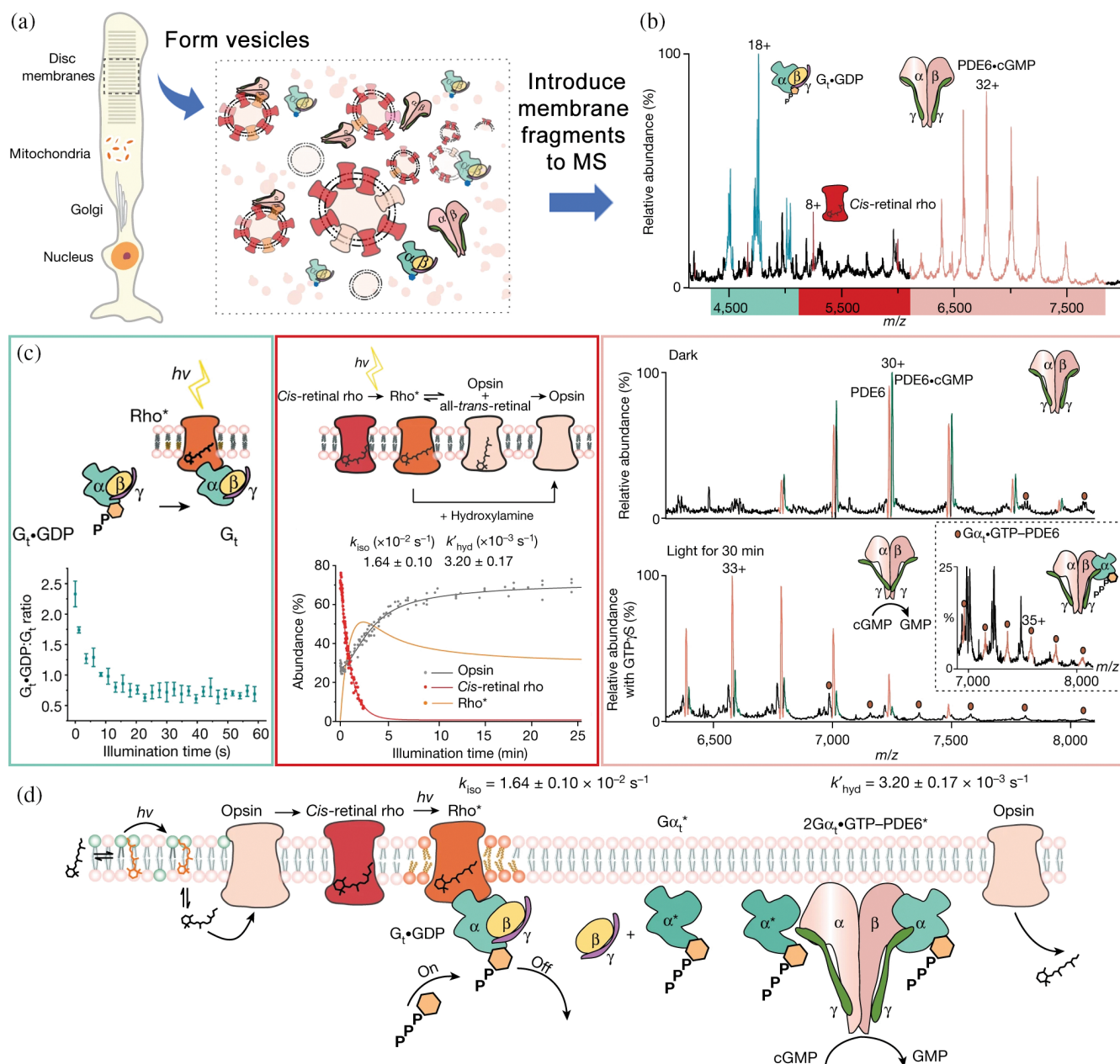
FIGURE 6 (a) Disc membranes are homogenized to form a heterogeneous distribution of vesicles that are introduced directly into the mass spectrometer. (b) Proteins along the signaling pathway were ejected and detected intact (red, cyan, and pink). (c) (left) The ratio of ground-state Gt•GDP (cyan) to intermediate apo-Gt decreases during the first 15 s after illumination. (middle) Monitoring the decay of cis-retinal rho (red line), the generation of opsin (gray line), and the change of rho* calculated over the illumination period (orange line). (right) Native mass spectra of PDE6 ejected from vesicles under dark conditions reveal the binding ratio and subpopulation (red circles). After exposure to light (right, bottom panel), the population of PDE6 bound to cGMP is reduced. (d) Schematic showing the rho* signaling cascade. Adapted with permission from Chen, Getter, et al. (2022).
