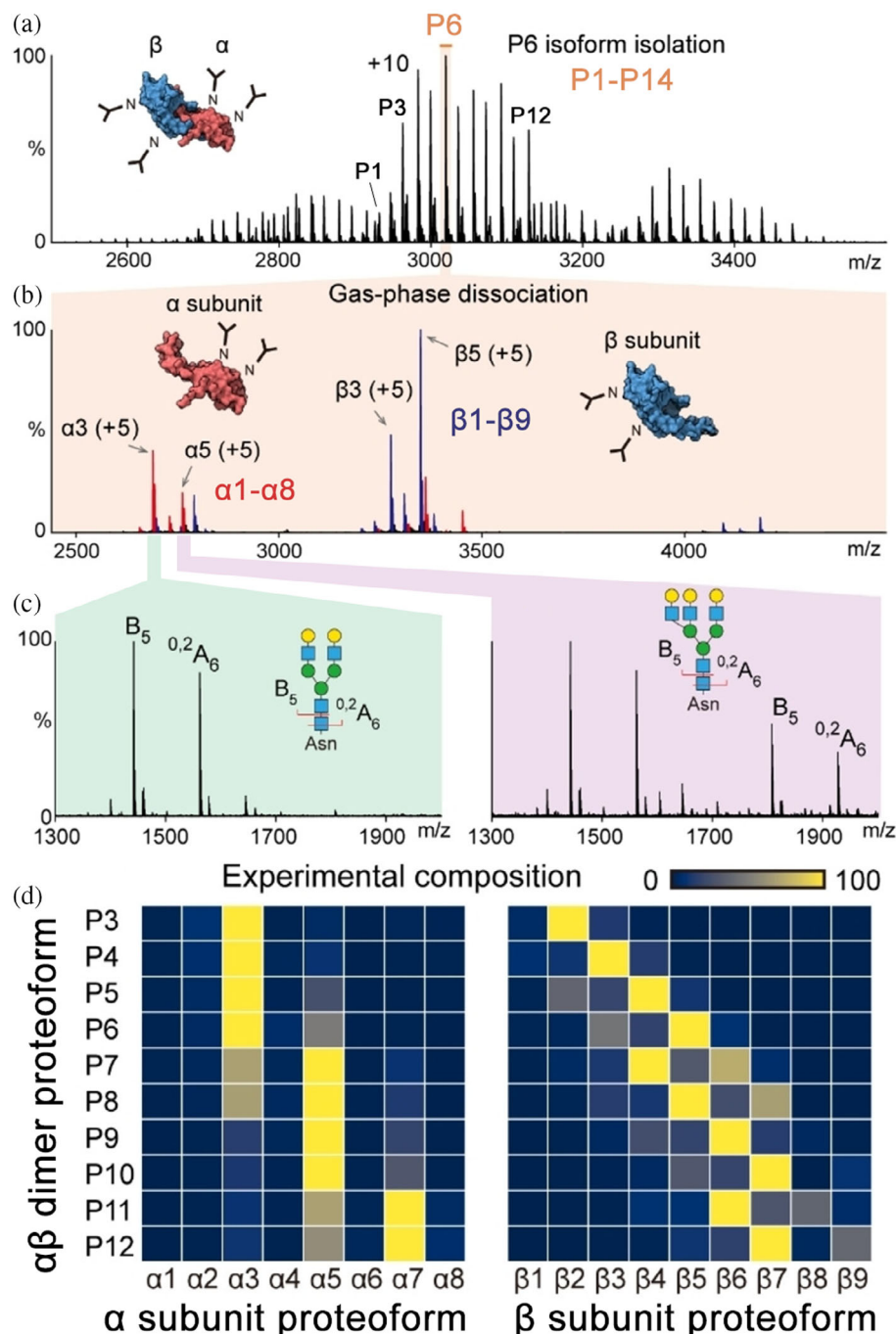
FIGURE 5 (a) Native top-down MS reveals detailed subunit proteoform composition of follitropin dimer. Among the 14 dimer proteoforms (P1–P14), P6 ( m/z 3019, charge state +10) was isolated for gas-phase dissociation. (b) Peaks in the MS/MS spectrum are annotated to the corresponding subunits ( \alpha subunits—red peaks with 8 proteoforms, \beta subunits—blue peaks with 9 proteoforms). P3–P12 proteoforms were further isolated and dissociated into \alpha and \beta subunits. (c) N-glycan composition of follitropin \alpha subunits. The released proteoforms \alpha 3 ( m/z = 2689, charge state +5) and \alpha 5 ( m/z = 2762, charge state +5) were selected and further fragmented. N-glycan fragments in the low mass range informed the difference in glycan structures in the two proteoforms. (d) Heatmap for experimentally measured \alpha/\beta subunit compositions of follitropin dimers (P3–P12). Adapted with permission from Wu and Robinson (2022).
