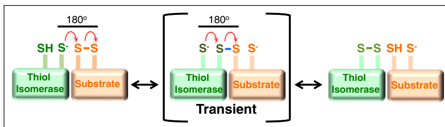
Figure 2. Mechanism of oxidoreductive cleavage by thiol isomerases. The reduced thiol isomerase aligns with a substrate that contains a disulfide bond such that the free thiolate forms an 180° angle with the vector of the disulfide. A second-order nucleophilic substitution S_N2 -type reaction then occurs in which the active site sulfur ion nucleophile of the thiol isomerase attacks the adjacent sulfur atoms of the disulfide bond. 74 This nucleophilic substitution results in a transient mixed disulfide (blue). The mixed disulfide spontaneously decomposes, resulting in the formation of a disulfide bond in the thiol isomerase and reduction of the disulfide bond in the substrate.
