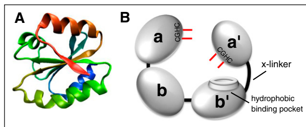
Figure 1. The architecture of thiol isomerases. Thiol isomerases consist of tandem domains containing a thioredoxin-fold. (A) The structure of the thioredoxin-fold. 7 (B) PDI is formed from 4 tandem domains containing thioredoxin-like folds that assume a U-shape. The 2 catalytic domains (a and a') contain the CGHC motifs that contain the catalytic cysteines (shown in red). The catalytic cysteines face one another and are responsible for oxidoreductive activities. The substrate binding domains (b and b') form the bottom of the U-shape. The b' domain contains a hydrophobic binding pocket that is primarily responsible for substrate binding. The b' and a' domains are connected by a flexible 19-amino-acid peptide termed the x-linker.
