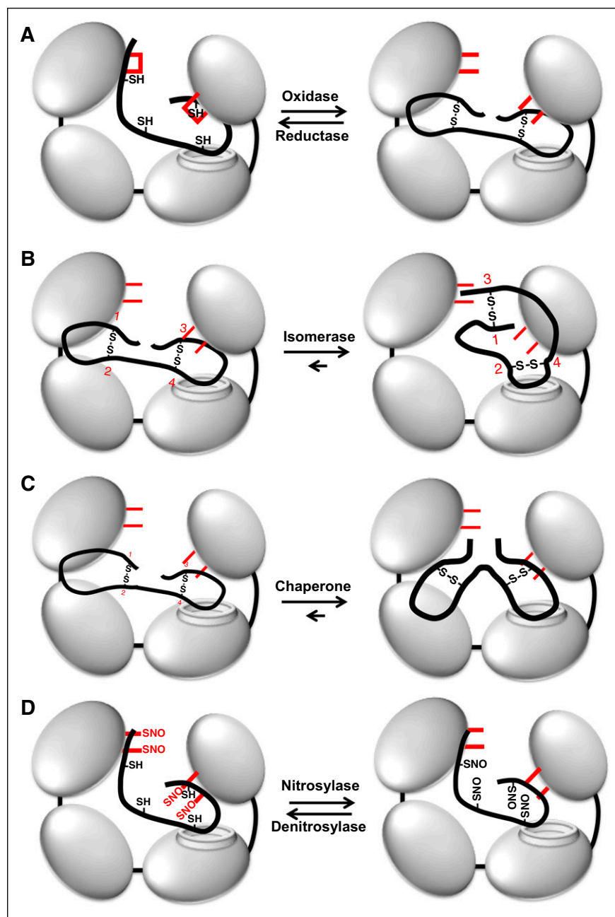
Figure 3. Multiple functions of PDI. (A) PDI is an oxidoreductase that can both form (oxidase) and cleave (reductase) disulfide bonds. Active site cysteines are shown in red. Note that the catalytic cysteines are either reduced or oxidized during these processes. (B) Through its oxidoreductase activity, PDI acts as an isomerase changing disulfide bond patterns within a protein. In this example, PDI modifies disulfides formed between cysteines 1-2 and 3-4 into disulfides formed between 1-3 and 2-4 (numbering in red). Note that there is no net change in the redox state of the catalytic cysteines on PDI. (C) PDI can act as a chaperone, modifying the conformation of a protein independent of its oxidoreductase and chaperone activities. The redox state of the catalytic cysteines is unchanged. (D) The active site cysteines within PDI can also become S -nitrosylated. PDI can then transfer NO to substrates, thus acting as a nitrosylase. PDI can also act as a denitrosylase, removing NO from substrates. S -nitrosylation typically inactivates substrates, whereas denitrosylation activates substrates.
