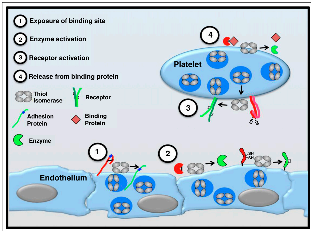
Figure 7. Functional consequences of thiol isomerase-mediated disulfide bond modifications. Thiol isomerases are secreted from platelets and endothelium following cell activation and mediate modifications of functional disulfide bonds in multiple substrates. Several categories of modifications are observed. (1) Exposure of binding sites in adhesion proteins. Cleavage of disulfide bonds can reveal cryptic binding sites such as RGD sequences (shown in blue) enabling a nonbinding adhesion protein (red) to adhere to binding partners on the cell surface (green). Thrombospondin is an adhesion protein that is modified in this manner. 53 (2) Activation of enzyme function. Functional disulfide bond cleavage could also expose an encrypted active site within an enzyme or modify its conformation, converting the enzyme to a more active conformation. Conversely, formation of a disulfide bond could activate an enzyme or coenzyme (eg, tissue factor). 65,66,93 (3) Receptor activation. Disulfide bond shuffling could contribute to the formation or stabilization of the active conformation of cell surface receptors (eg, \alpha_{IIb}\beta_3 ). 47,75 (4) Release from binding protein. Cleavage of a disulfide bond could release a protein from its binding partner, thereby activating the protein (eg, TGF- \beta ). 94
