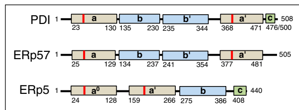
Figure 6. Domain structures of vascular thiol isomerases. (A) The domain structures of thiol isomerases with known activity in thrombus formation (PDI, ERp57, and ERp5) are shown. Catalytic domains (tan), binding domains (blue), and c domains (green) are indicated. The location of the CGHC motif is indicated in red. Numbers indicate the amino acid position in the mature protein.
