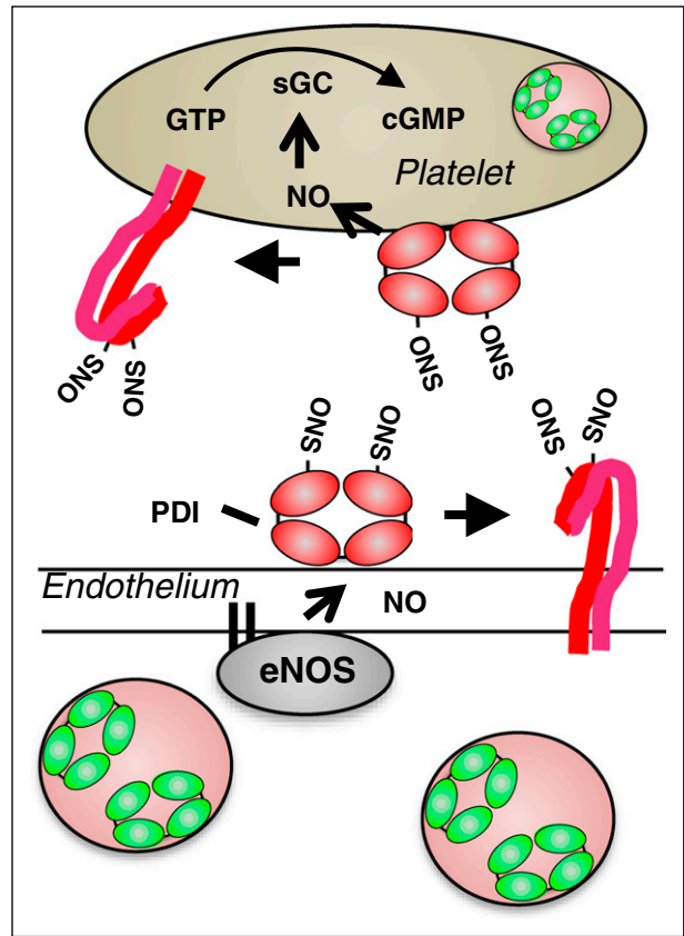
Figure 5. Proposed model for the role of PDI in regulating vascular NO activity. In the quiescent vasculature, when NO levels are high, PDI may be S-nitrosylated. Endothelial SNO-PDI could transfer NO to surface proteins, thereby inhibiting their activity, or transfer NO intracellularly. Intracellular NO could bind to guanylyl cyclase, stimulating the generation of cGMP and contributing to the platelet quiescence.
