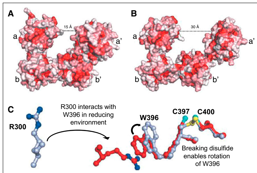
Figure 4. Redox sensitivity of PDI. (A) In a reducing environment, PDI assumes a compact structure characterized by a 15-Å distance between the a and a' domains. (B) In an oxidizing environment, the distance between the a and a' domain increases to 30 Å. The increase in distance results from loss of interactions between the b' and a' domains that allows movement of the x-linker and a' domains. Adapted from Wang et al. 23 (C) In a reducing environment, the disulfide bond between C397 and C400 is broken, enabling the rotation of W396. This rotation positions W396 so that it can interact with R300. The interaction between W396 and R300 brings the a' domain in closer proximity to the b' domain, facilitating additional interactions that lead to a more compact structure. Adapted from Wang et al. 23
