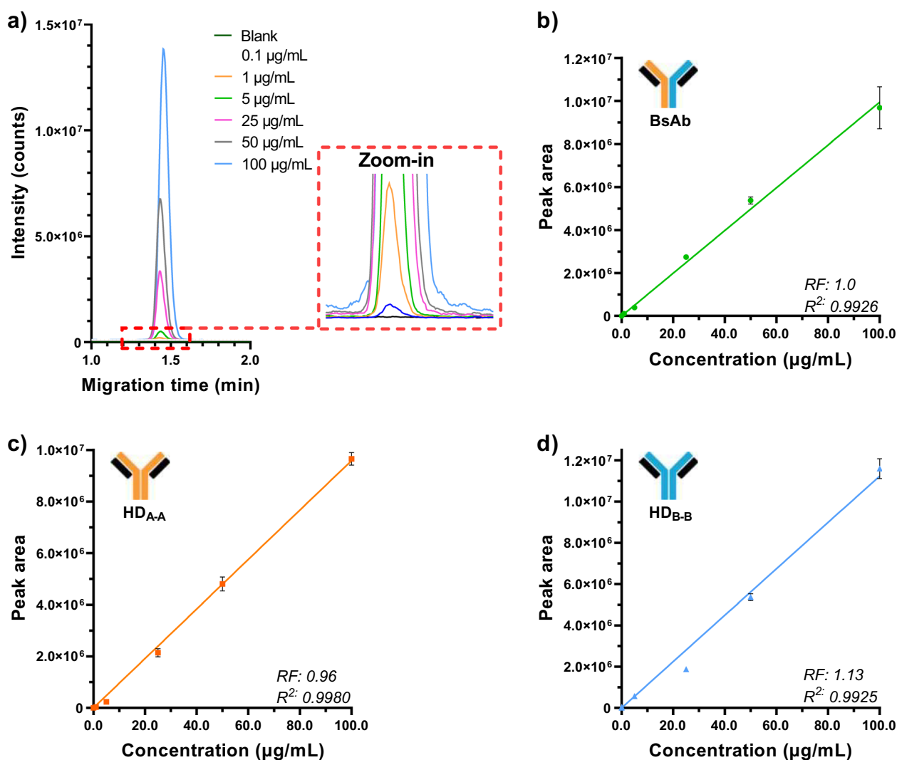
Fig. 3 a Overlay and zoom-in of seven TIEs obtained during MCE-MS of a blank diluent and BsAb solutions with concentrations ranging from 0.1 to 100 µg/mL using the high-throughput MCE-MS method. b–d Calibration curves (peak area vs. injected concentration)
