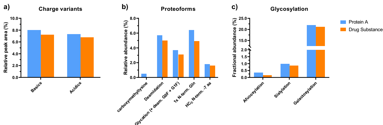
Fig. 8 Bar graphs showing the a peak area (%) of the basic and acidic charge variants, b the relative abundance (%) of the charge-migrating proteoforms, and c the levels (%) of afucosylation, sialylation, and galactosylation, obtained with the high-resolution MCE-MS method
