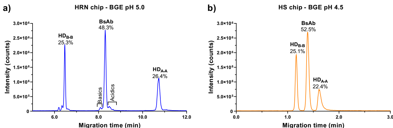
Fig. 2 BPEs obtained by MCE-MS analysis of an HD A-A -BsAb-HD B-B mixture (spiked ratio, 20:60:20) using a a 22-cm channel HRN chip and a BGE pH of 5.0 or b a 10-cm channel HS chip and a BGE pH of 4.5. The peaks of basic and acidic charge variants of the BsAb are indicated in a . Mass spectra of the observed peaks are depicted in Fig. S2. The measured fractional abundance of each Ab variant is denoted. Abbreviations used for peak assignment, see Fig. 1
