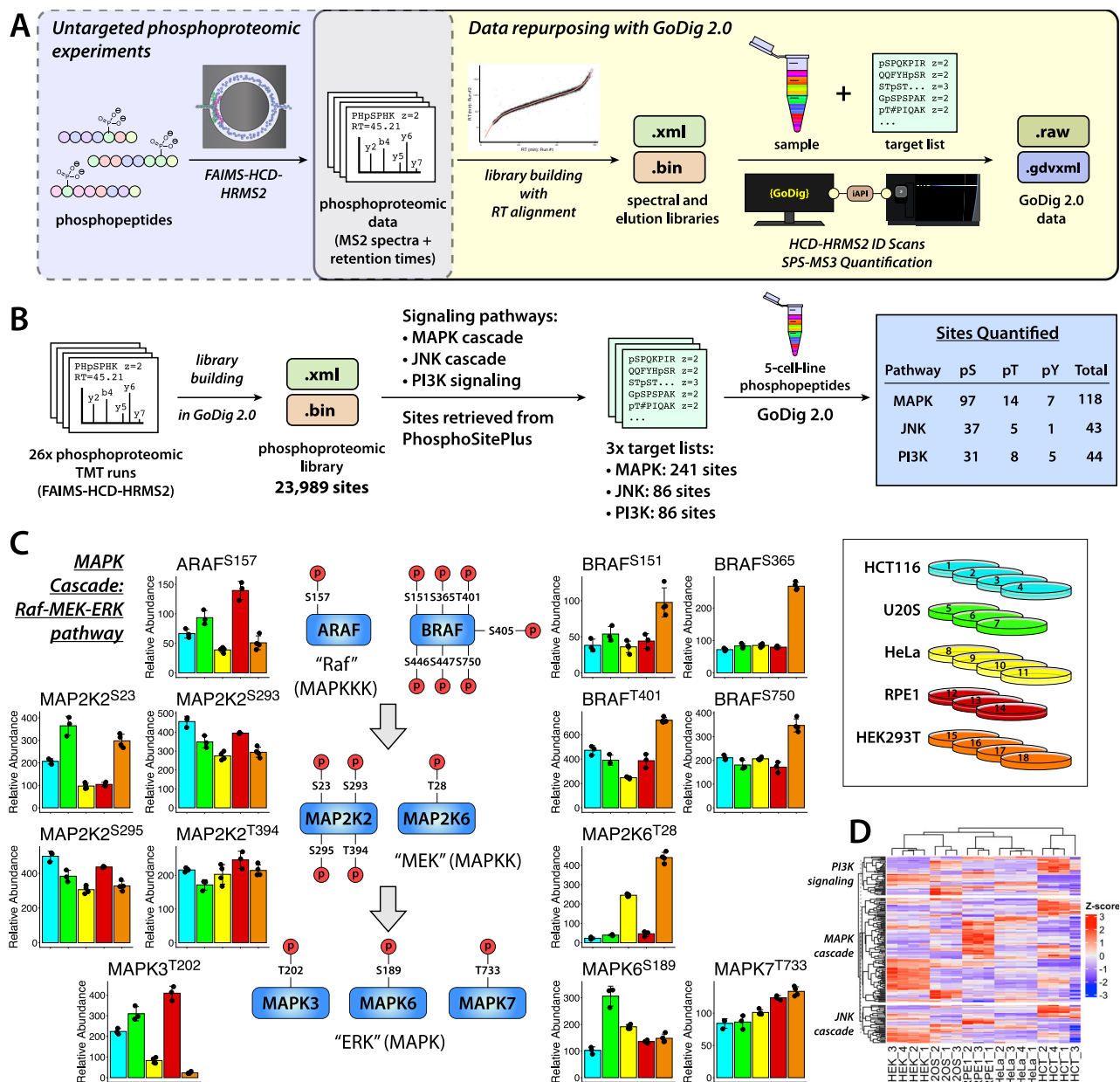
Fig. 4 | GoDig 2.0 enables the repurposing of existing phosphoproteomic data for streamlined targeted pathway analysis. A Data repurposing workflow depicted with phosphoproteomic data as an example. Previously acquired untargeted LC-MS/MS data, including PTM analyses, regardless of fragmentation mode, buffer gradient, or ion mobility-based separation, can be built into spectral and elution libraries using GoDig 2.0. B A three-pathway targeted phosphoproteomic experiment performed with GoDig 2.0. For each pathway, 3 priming runs and 1
