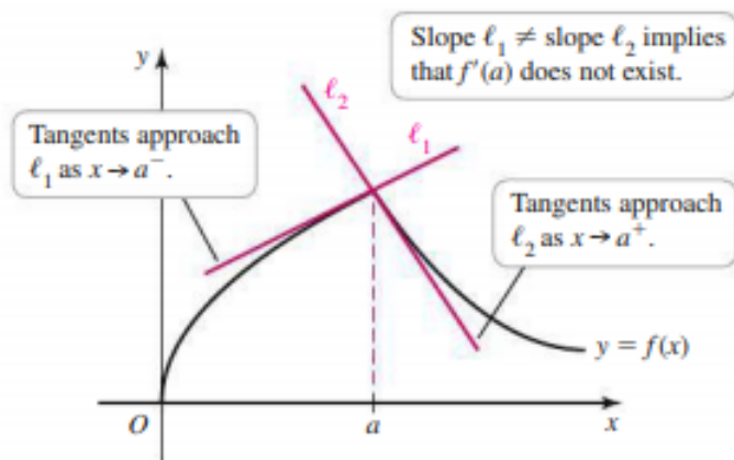
Figure 2: f has a corner at a
