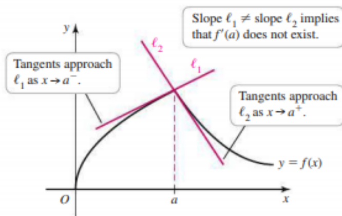
Figure 2: f has a corner at a
