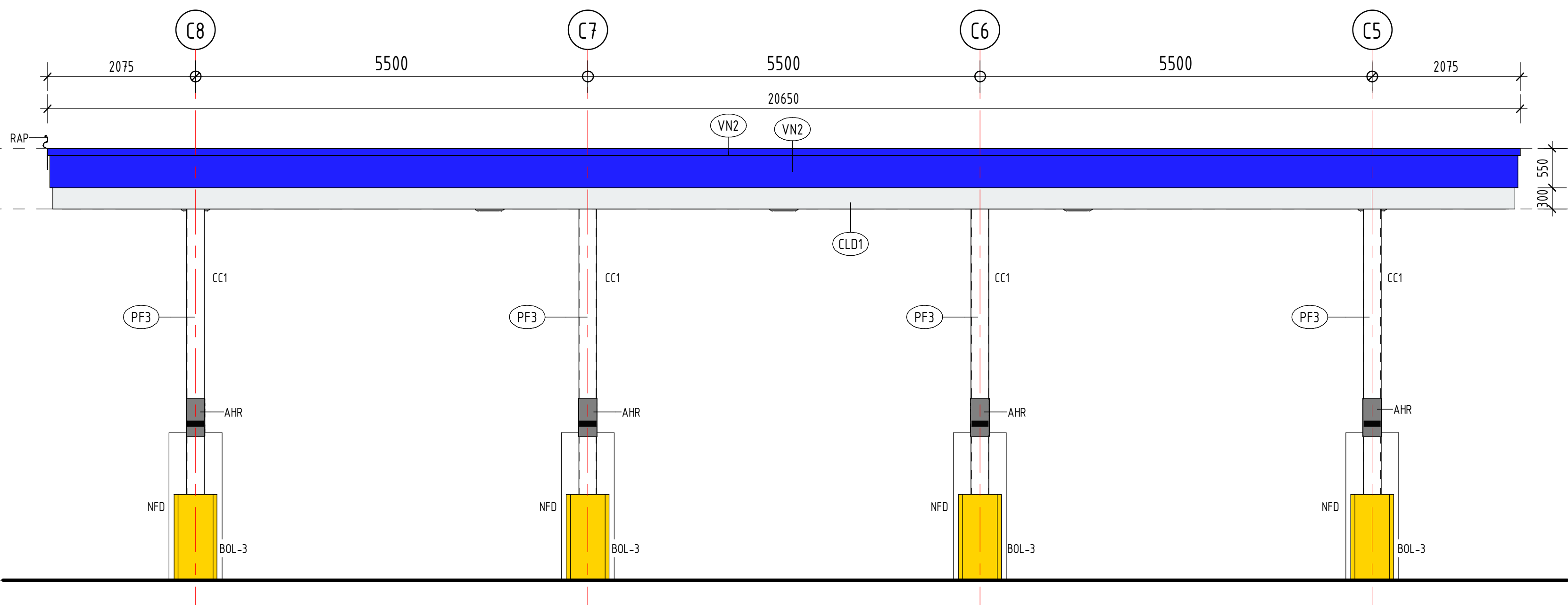
4 TRUCK CANOPY EAST ELEVATION 1 : 50
