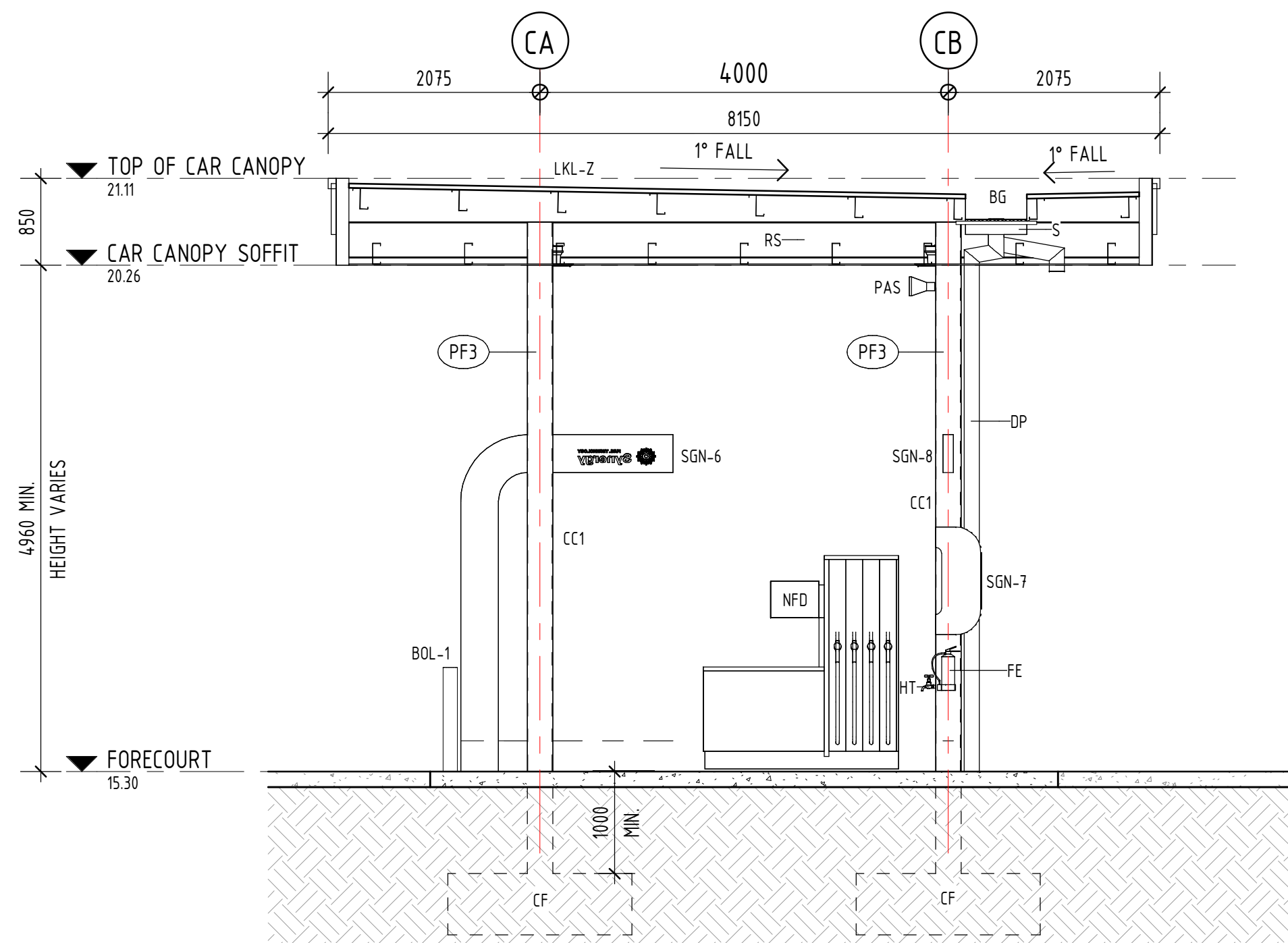
2 CAR CANOPY SECTION 2 1 : 50
