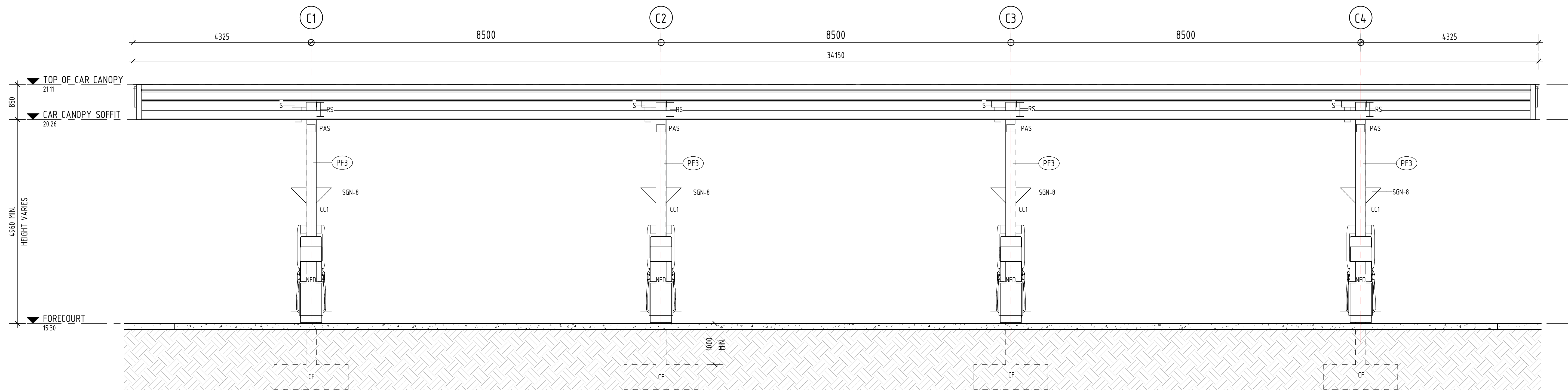
1 CAR CANOPY SECTION 1 1 : 50
