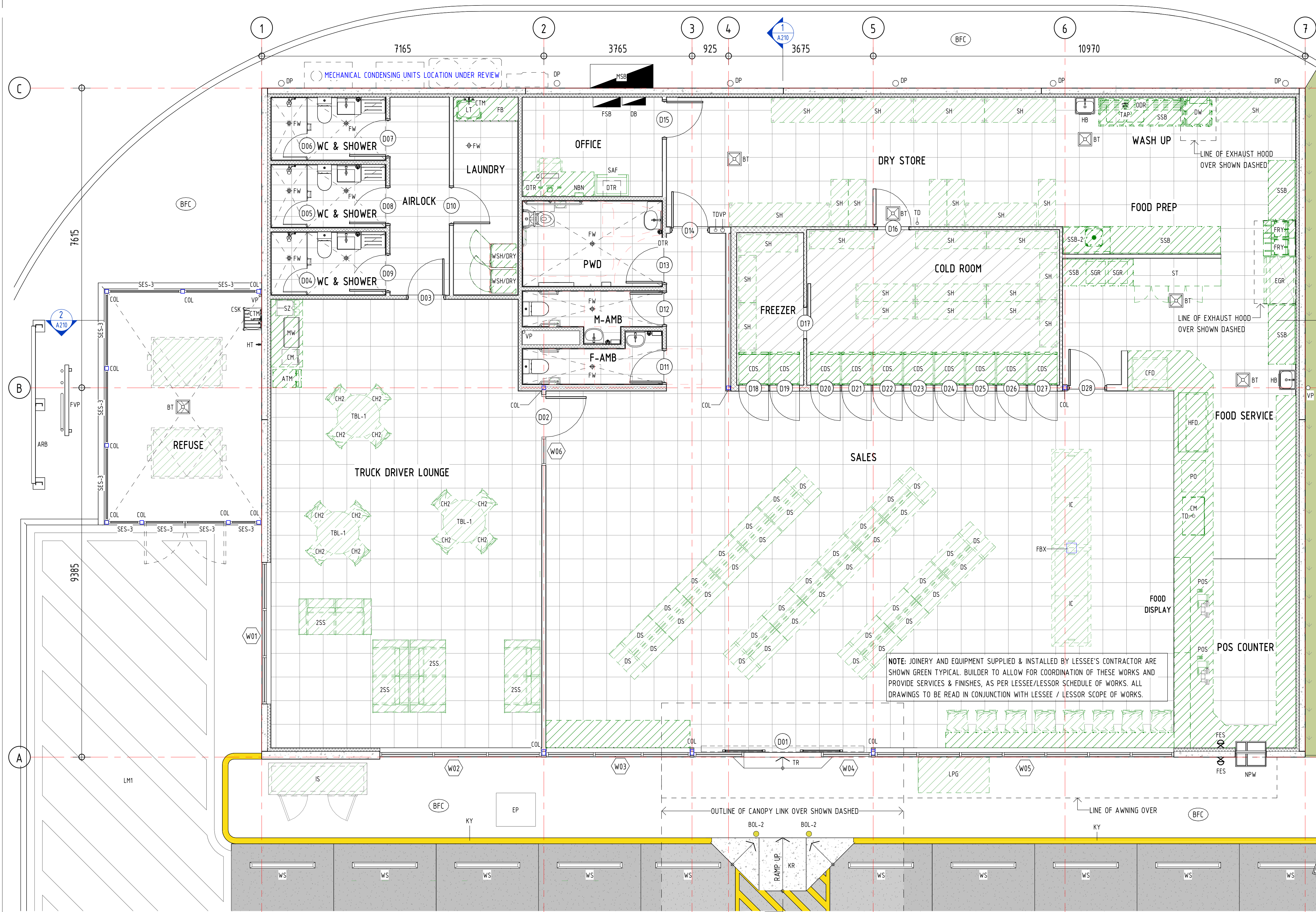
1 PROP. FLOOR PLAN 1:50
