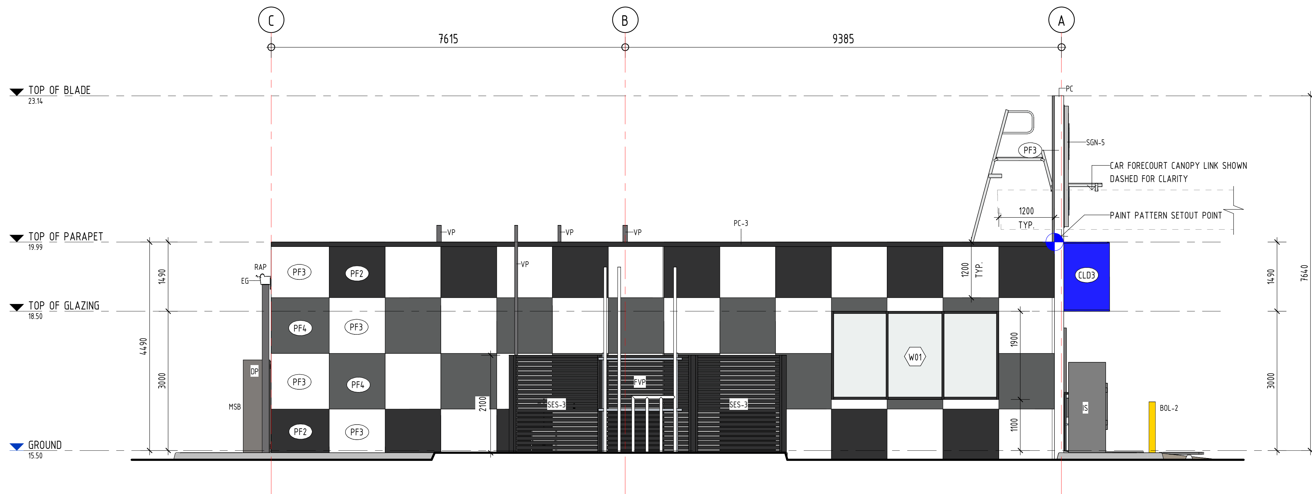
1 BUILDING ELEVATION NORTH 1 : 50
