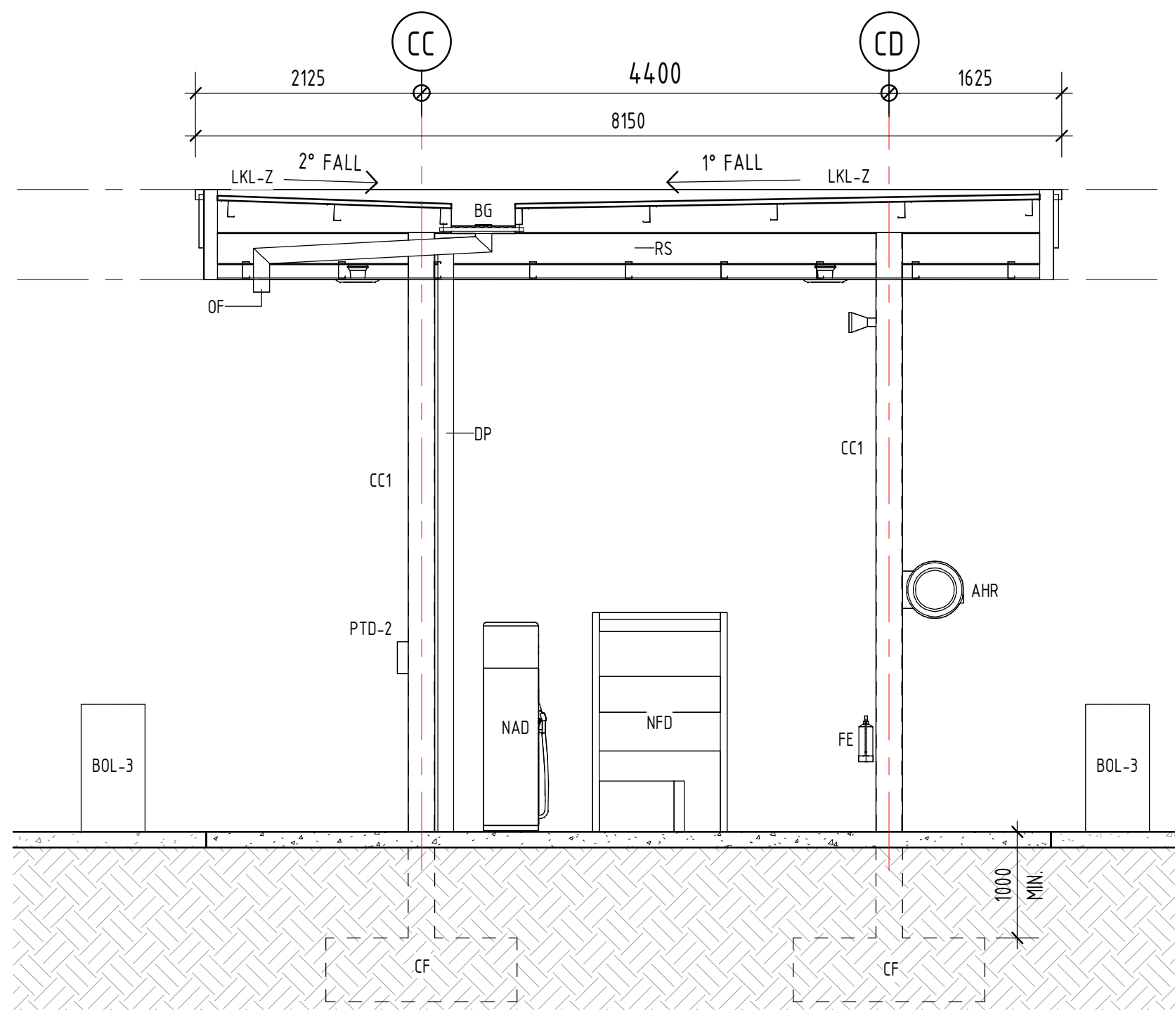
2 TRUCK CANOPY SECTION 2 1 : 50
