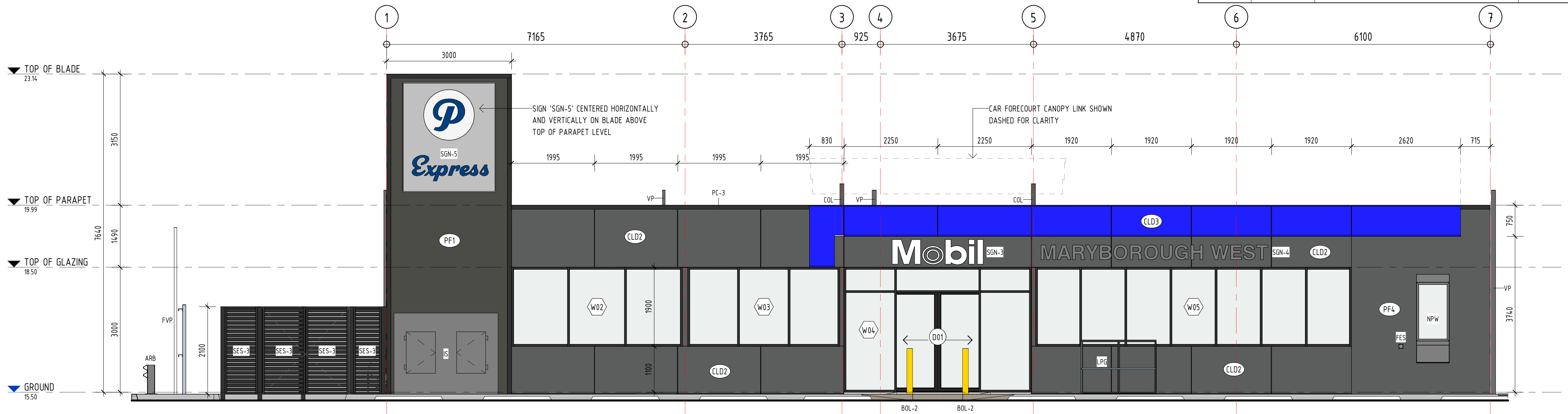
2 BUILDING ELEVATION WEST 1 : 50
