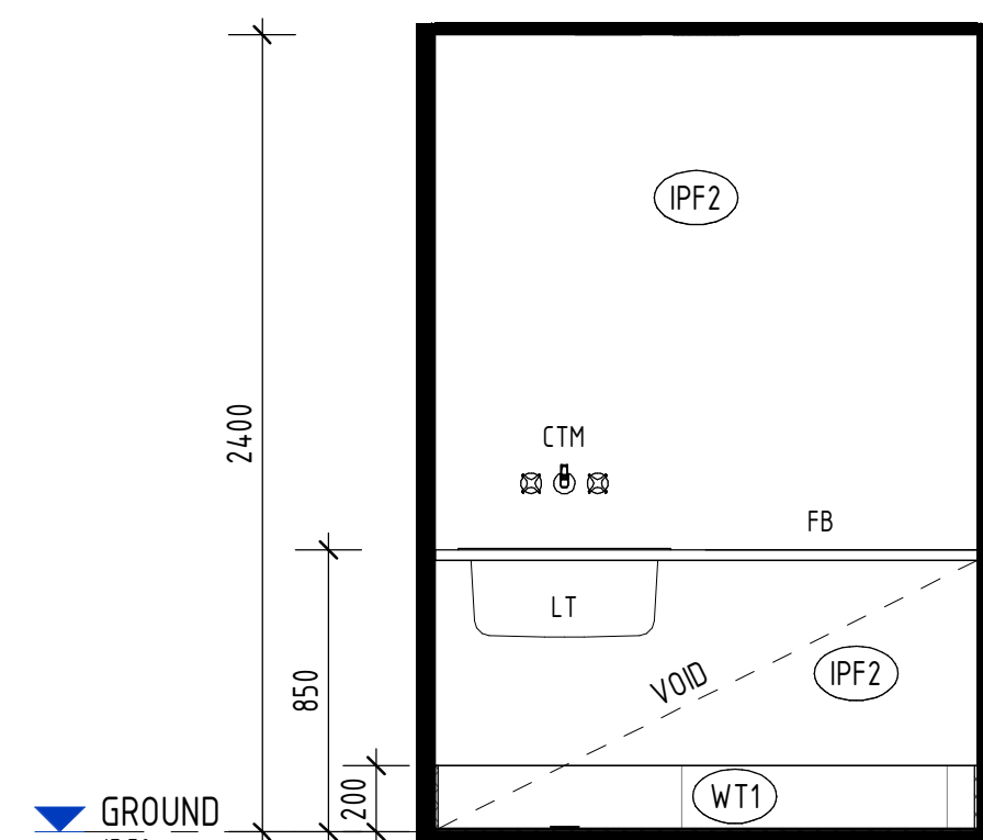
2 LAUNDRY - ELEVATION 1 1 : 25
