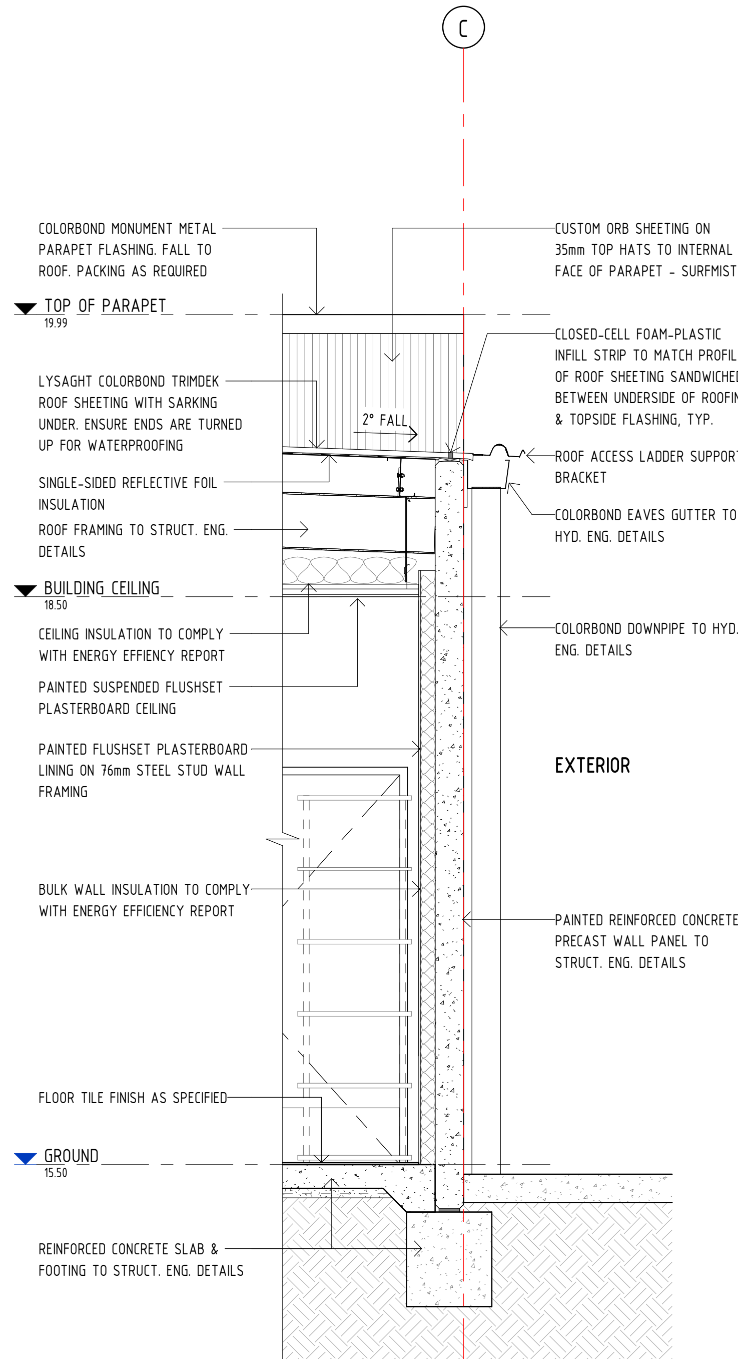
2 WALL SECTION 2 A210 1:20
