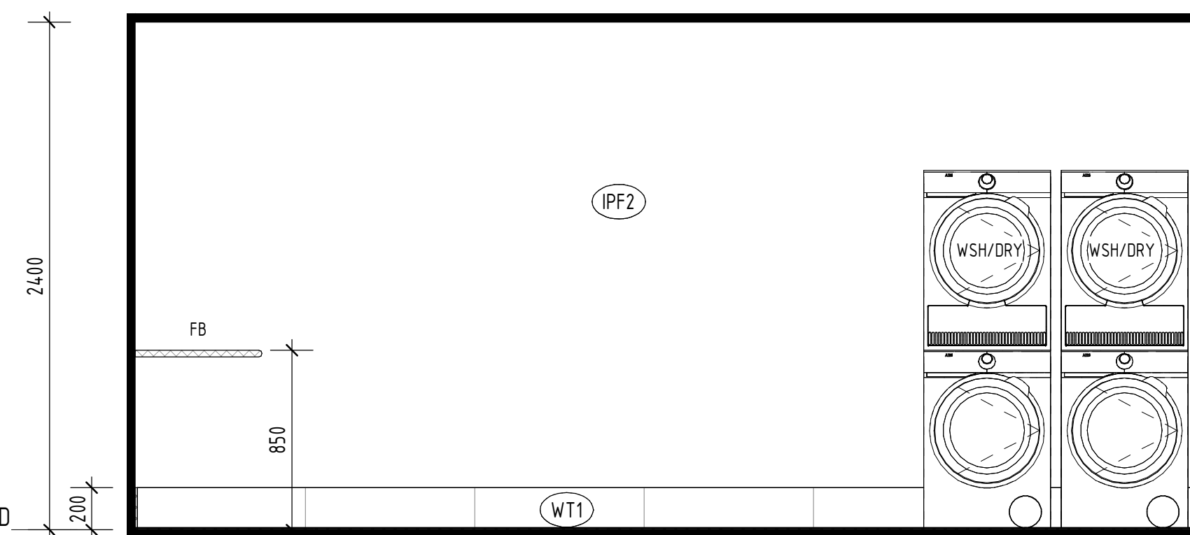
3 LAUNDRY - ELEVATION 2 1 : 25
