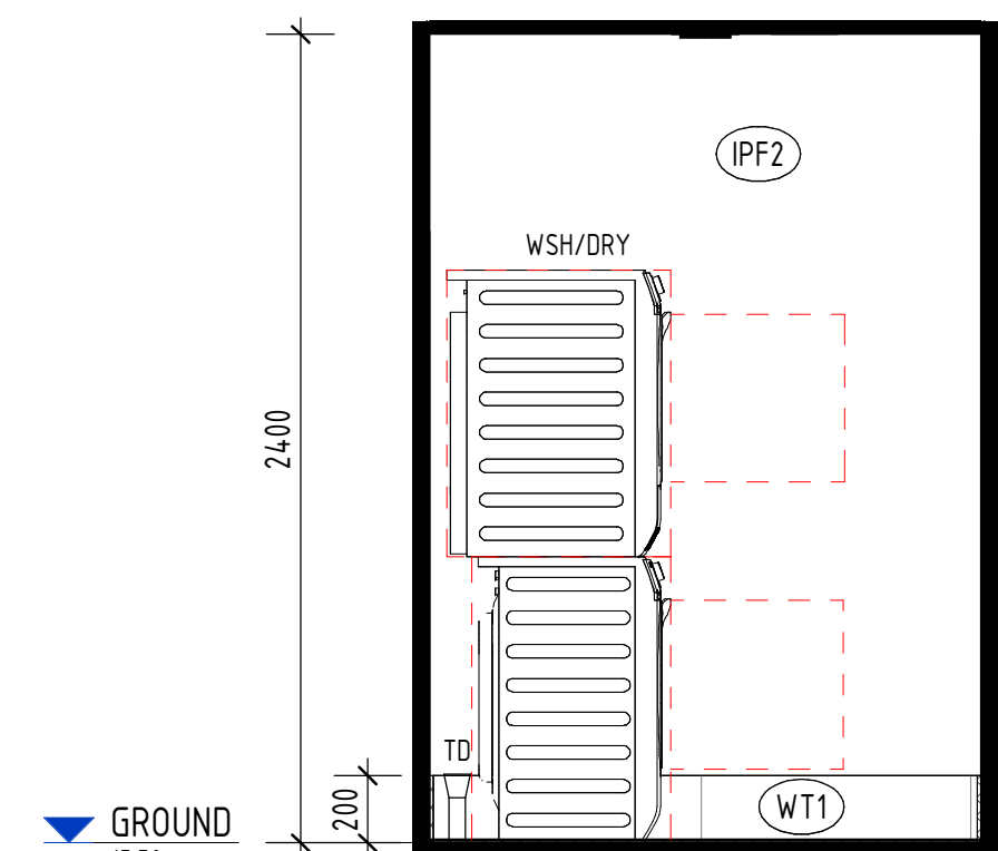
4 LAUNDRY - ELEVATION 3 1 : 25
