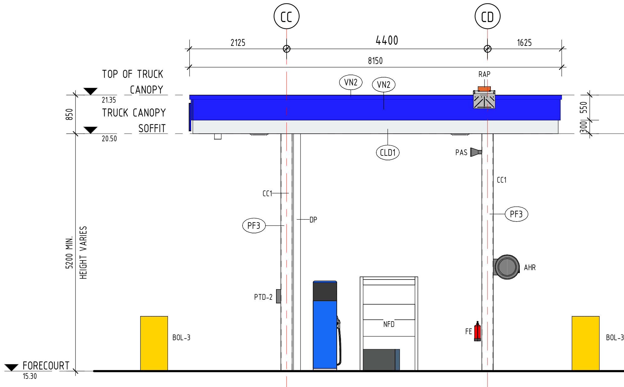
3 TRUCK CANOPY SOUTH ELEVATION 1 : 50
