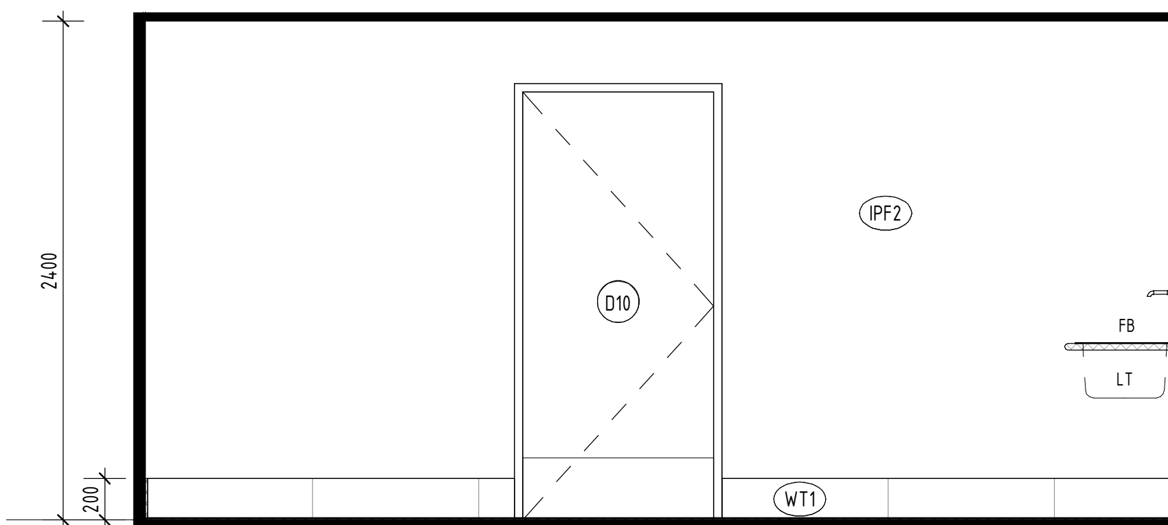
5 LAUNDRY - ELEVATION 4 1 : 25
