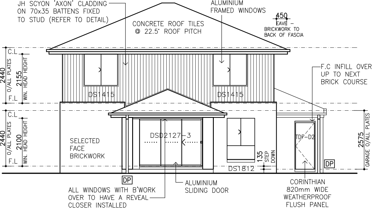
ELEVATION C
