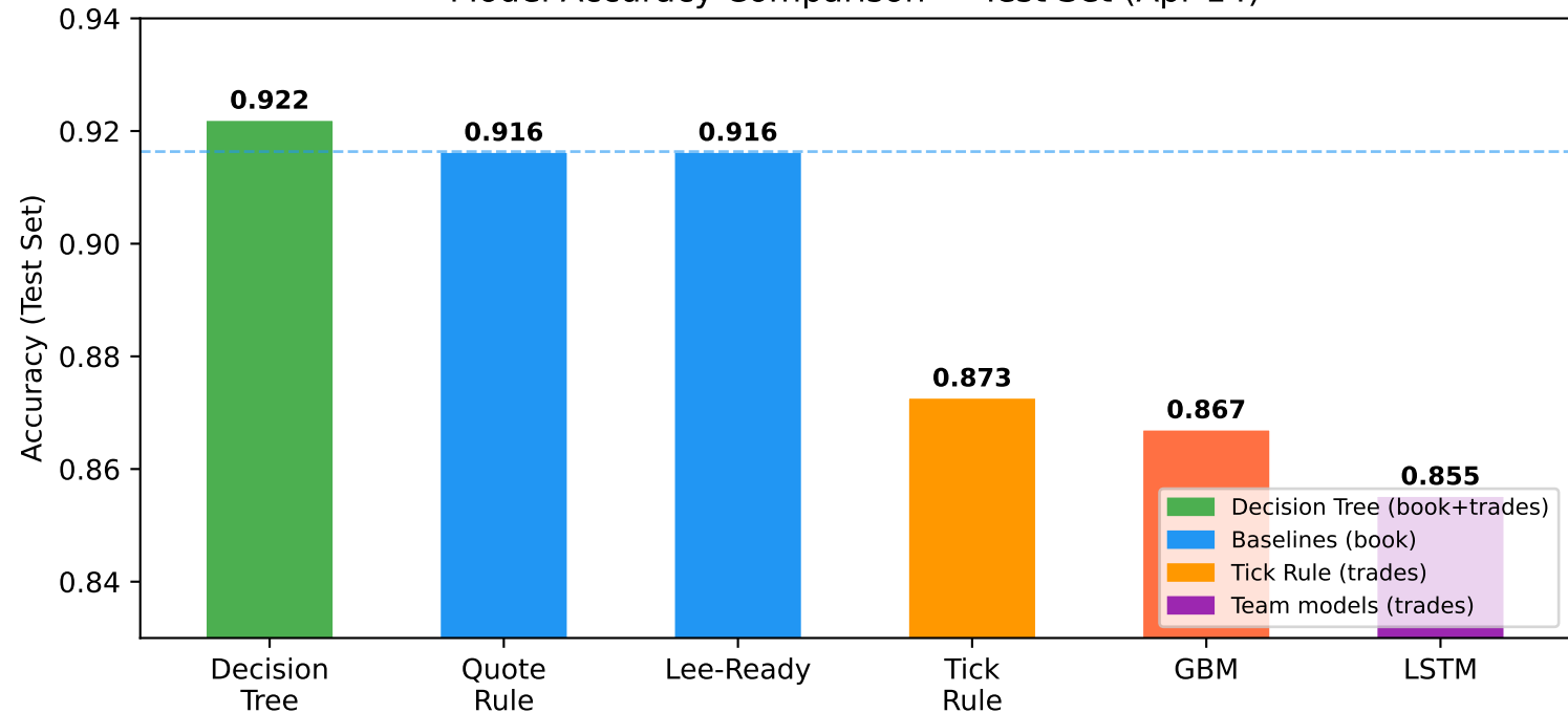
Model Accuracy Comparison — Test Set (Apr 14)
