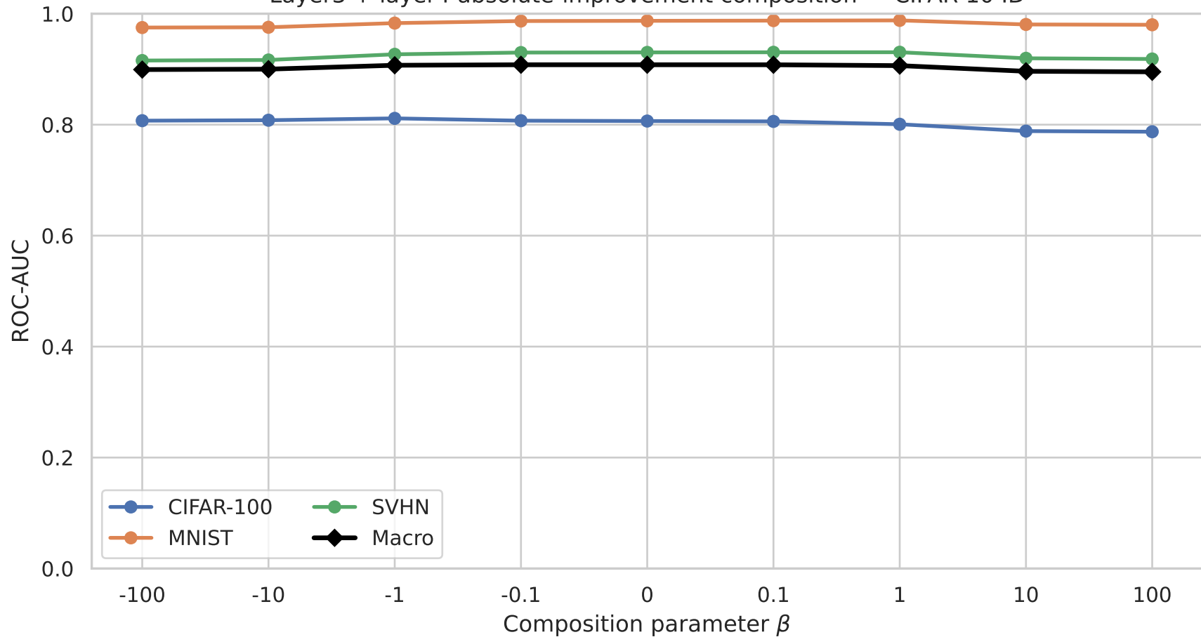
Layer3 + layer4 absolute-improvement composition — CIFAR-10 ID
