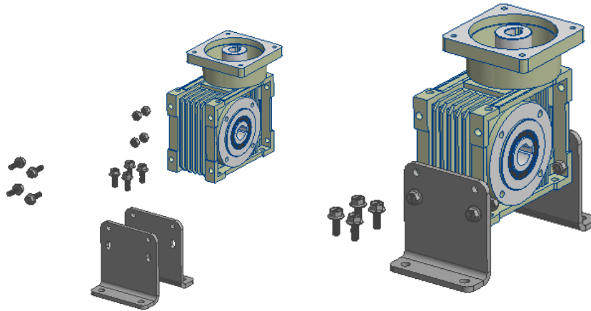
Figure 5.5a — L-bracket alignment and M6 × 20 flange bolt positions
