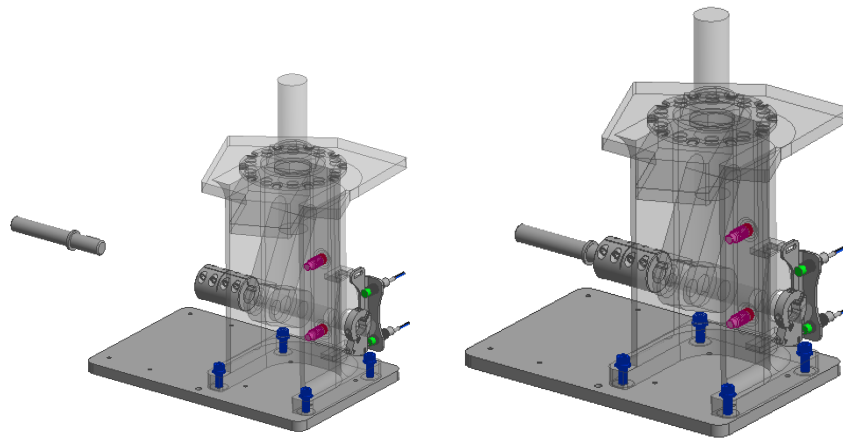
Figure 5.4b — Collar and shaft installation
