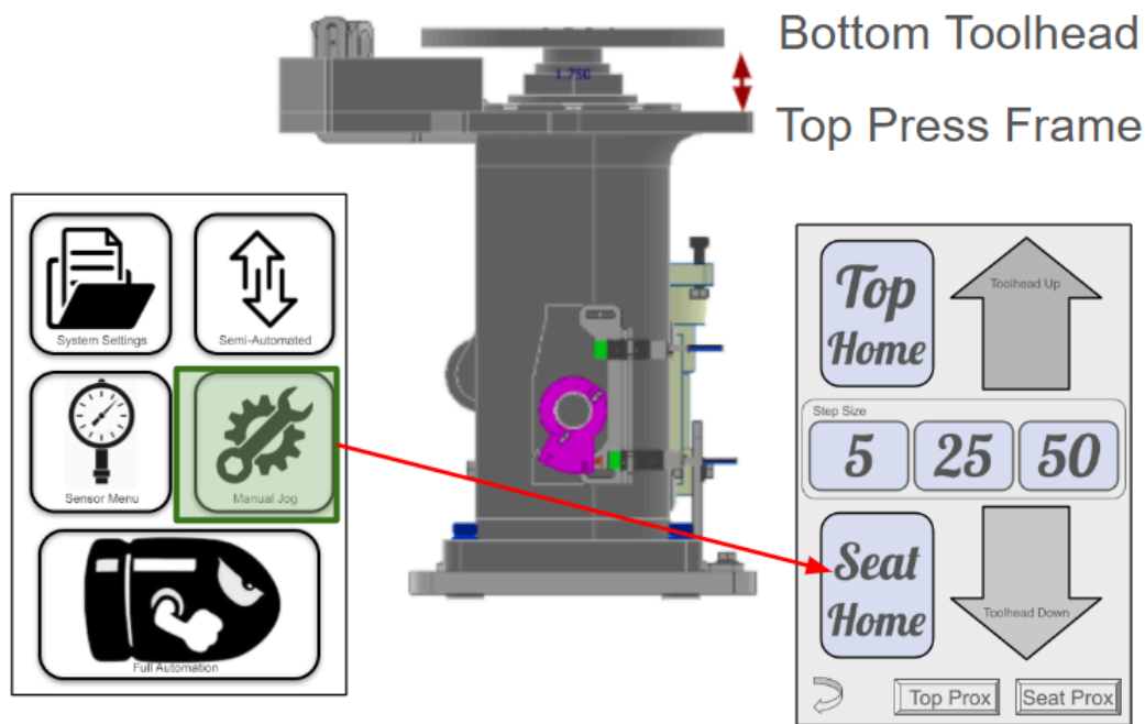
[ Figure 7.3a — Setting the bottom proximity sensor and measuring the gap ]
