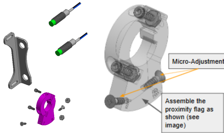
Figure 5.3a — Proximity flag assembly and M12 sensor installation
