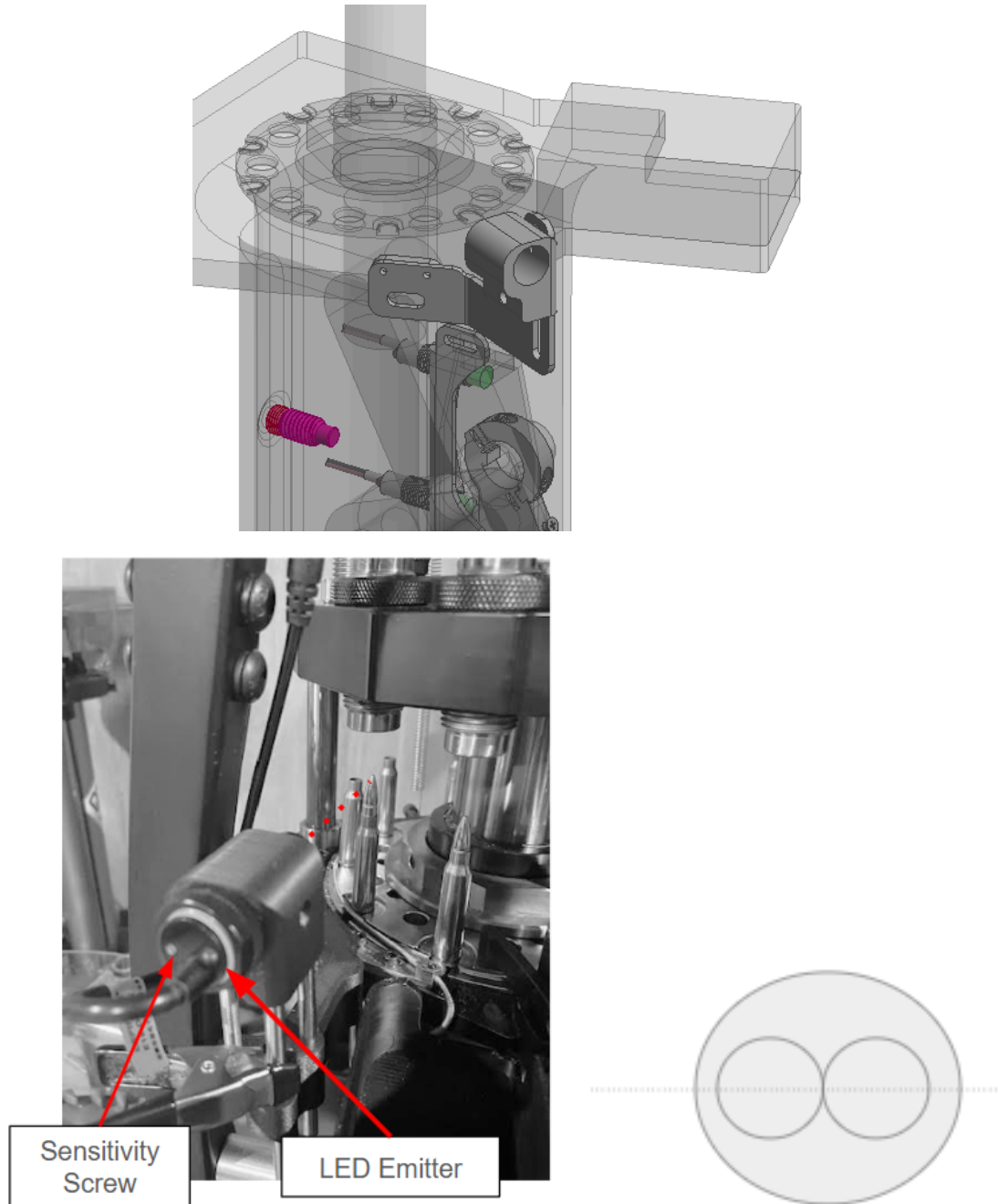
Figure 5.7a — Bullet sensor bracket mounting and alignment
