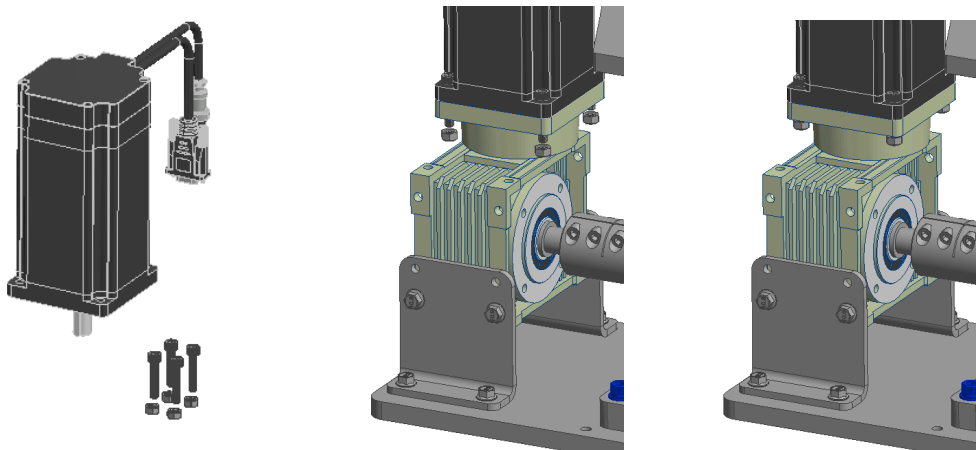
Figure 5.6b — NEMA 34 stepper motor installed into the gearbox
