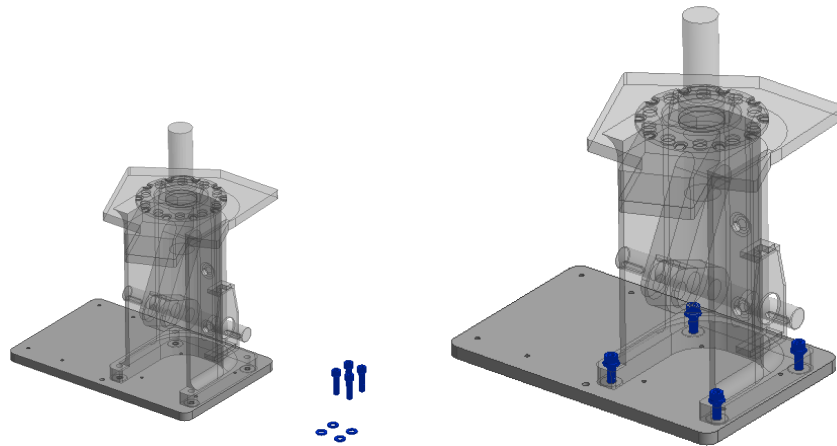
Figure 5.2c — Press aligned to base plate, M8 hardware installed loose
