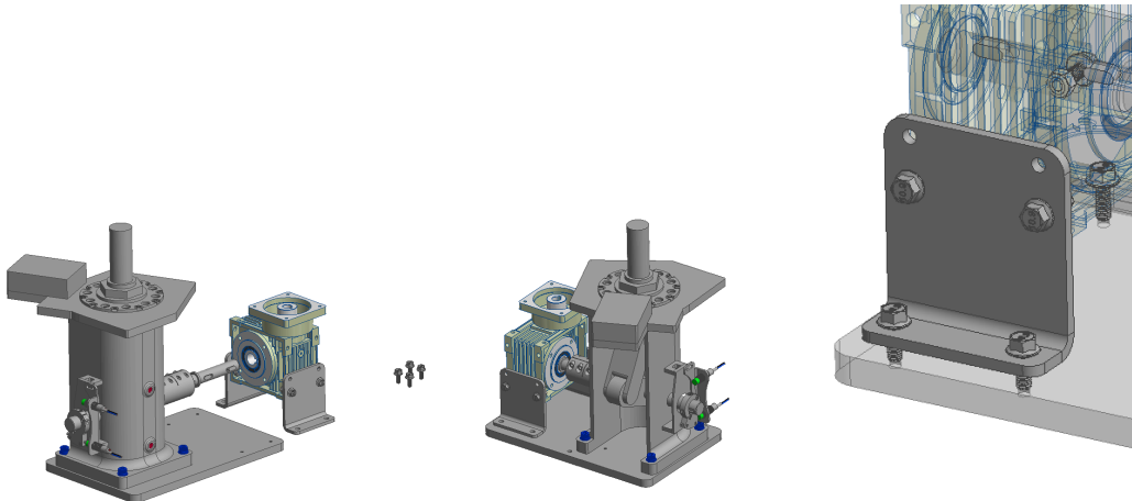
Figure 5.5b — Gearbox mounted to the L-brackets and base plate
