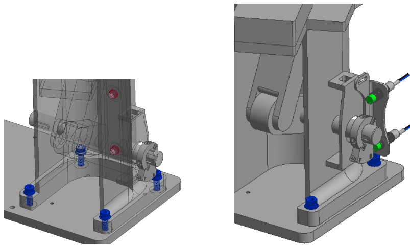
Figure 5.3b — Flag installed on keyed shaft, T and B markings facing outward
