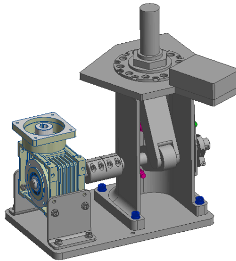
Figure 5.6a — Fully aligned assembly, ready to torque
