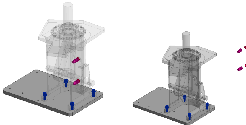
Figure 5.2d — Upper and lower rear hard stop locations
