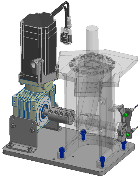
Figure 5.8a — Completed assembly
