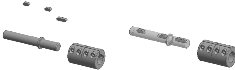
Figure 5.4a — Keys seated in the gearbox shaft
